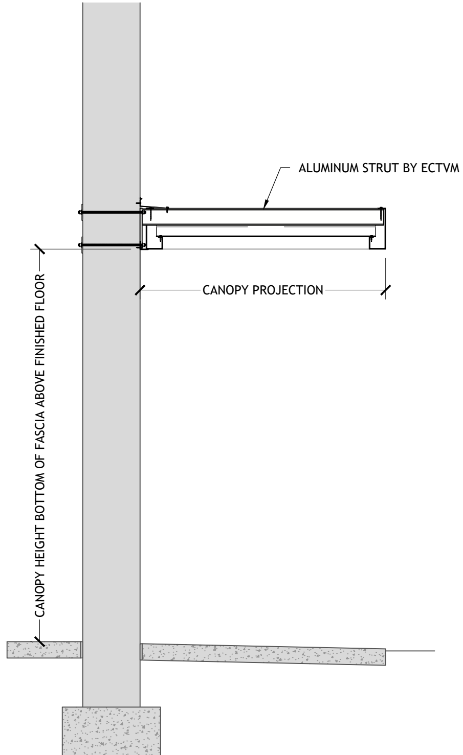
STRUT SUPPORT 10 INCH FASCIA FLUSH DECK
