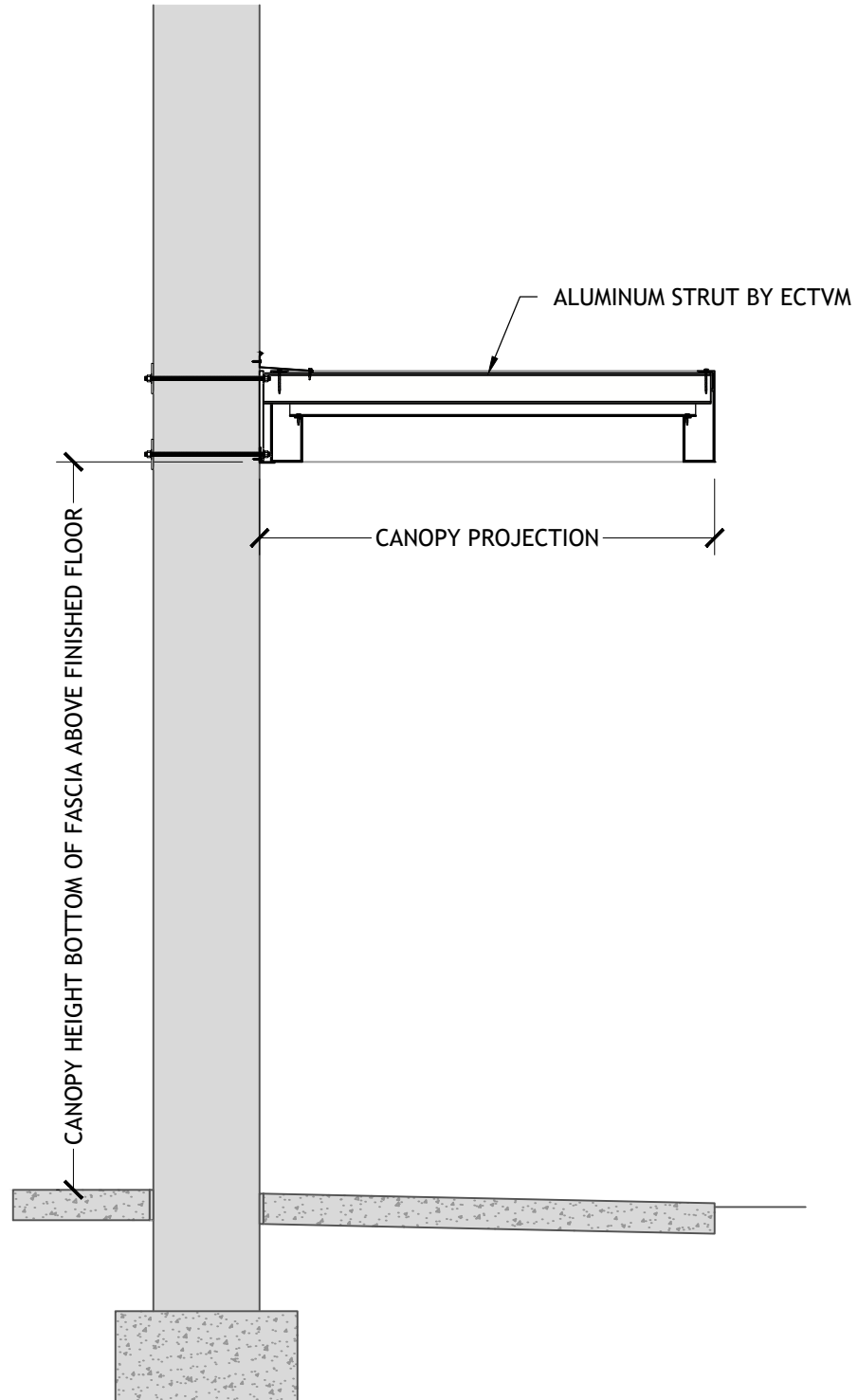
STRUT SUPPORT 12 INCH FASCIA FLUSH DECK
