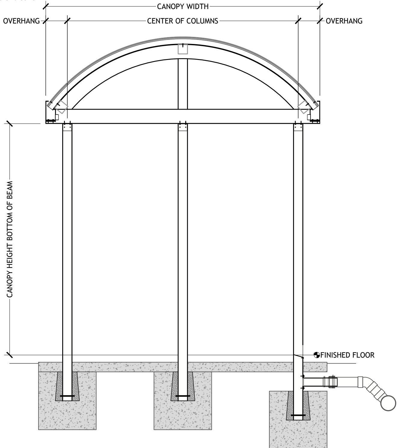
ARCHED TRUSS THREE POST PAN & CAP DECK UNDERGROUND DRAIN
