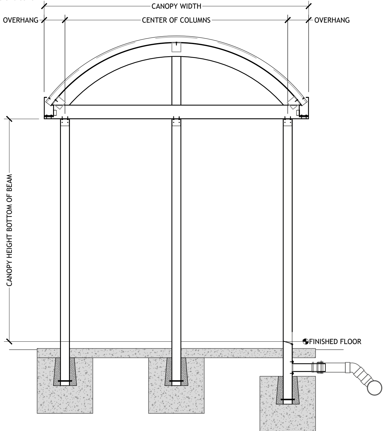
ARCHED TRUSS THREE POST FLUSH DECK UNDERGROUND DRAIN
