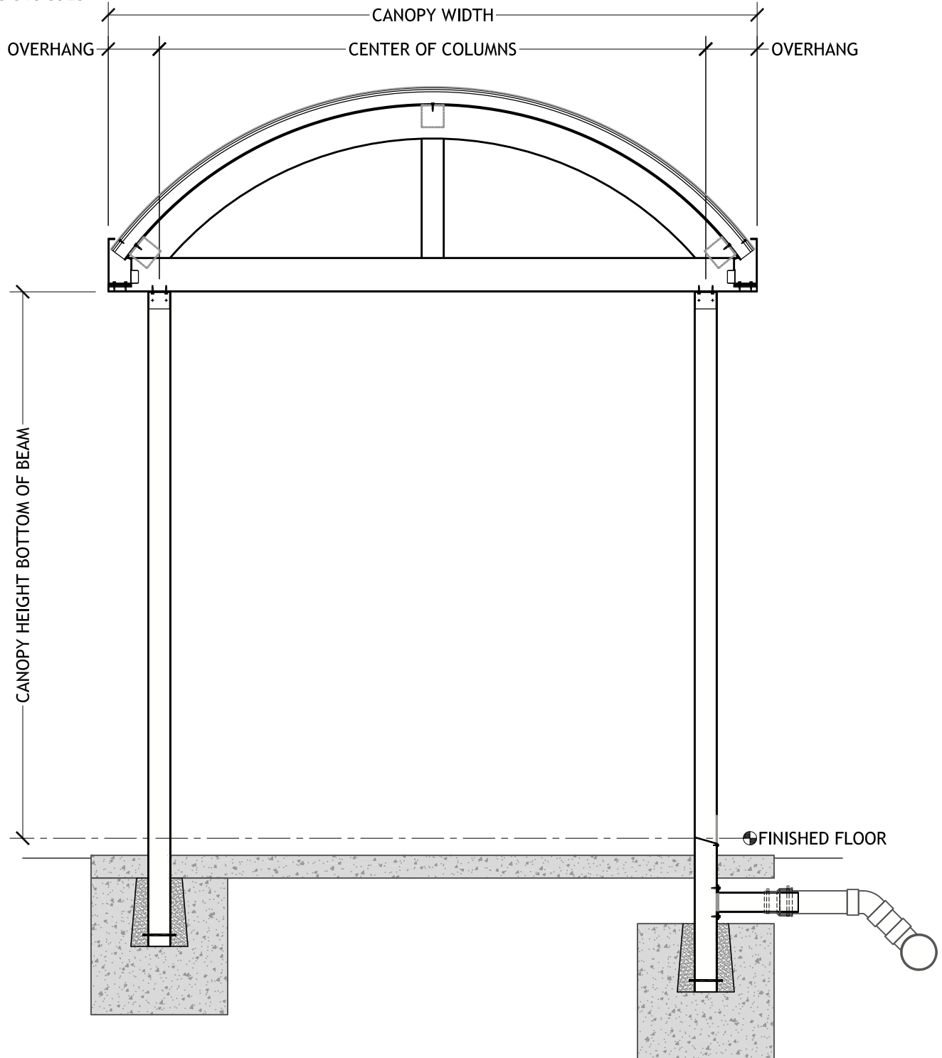
ARCHED TRUSS PAN & CAP DECK UNDERGROUND DRAIN
