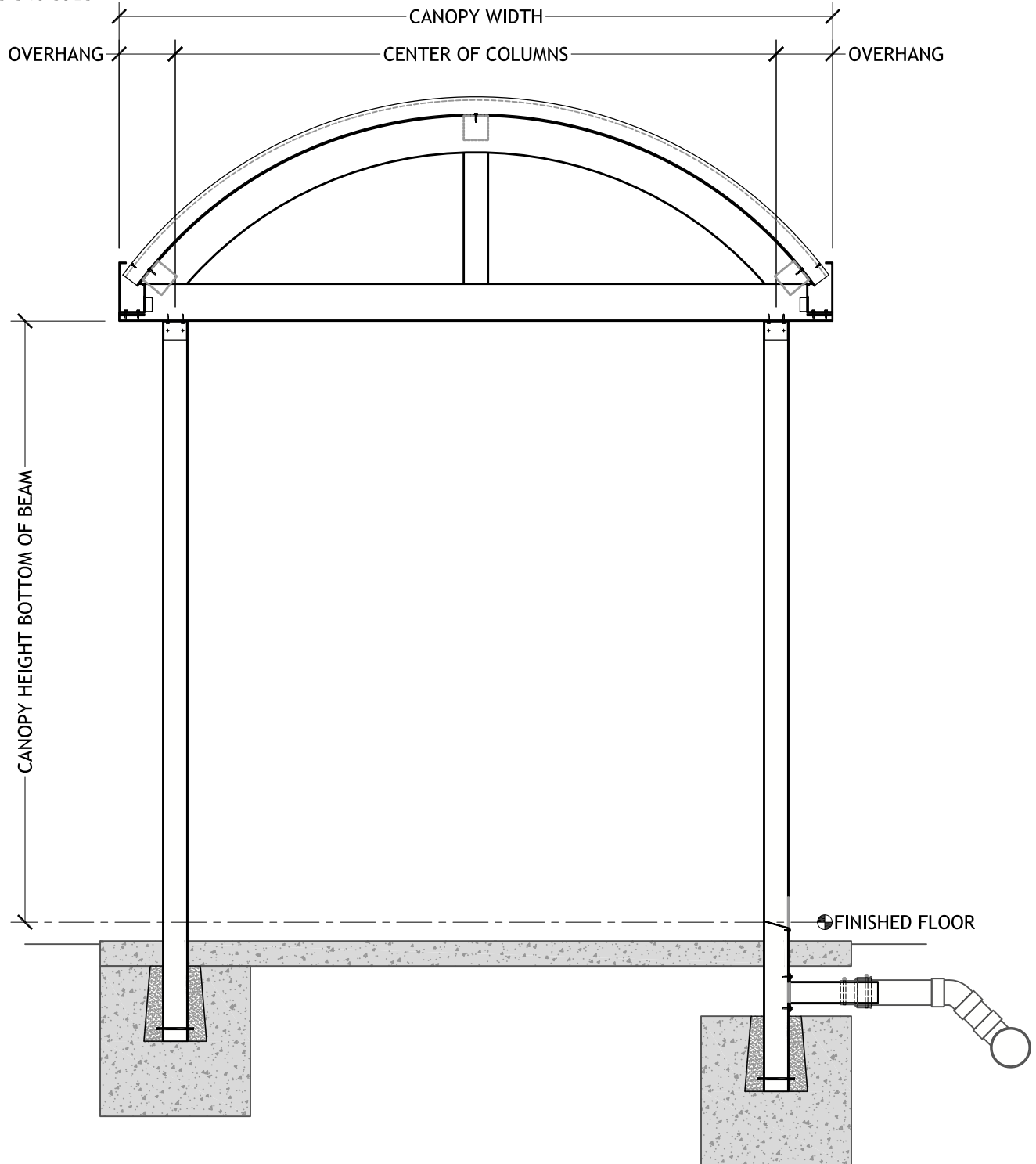
ARCHED TRUSS FLUSH DECK UNDERGROUND DRAIN
