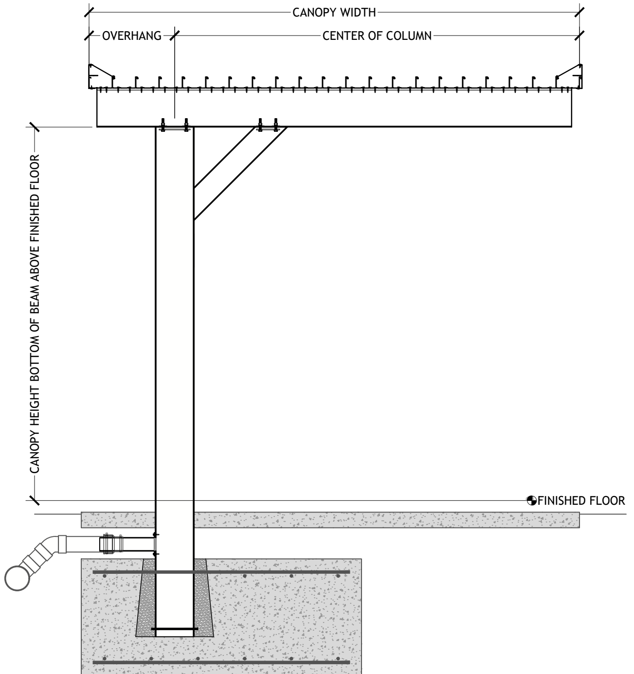
CANTILEVER BRACE LONG SPAN FLUSH DECK UNDERGROUND DRAIN
