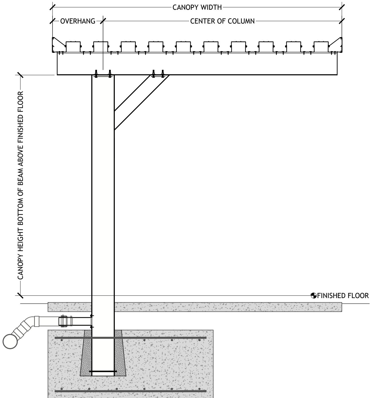
CANTILEVER BRACE LONG SPAN HIGH PAN & CAP DECK UNDERGROUND DRAIN
