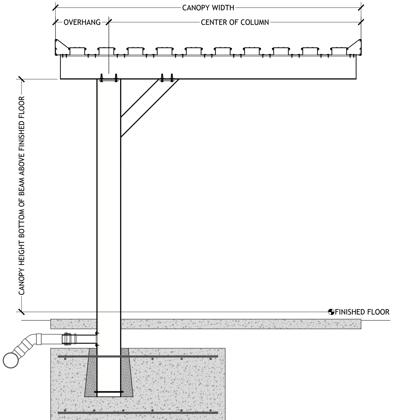
CANTILEVER BRACE LONG SPAN PAN & CAP DECK UNDERGROUND DRAIN
