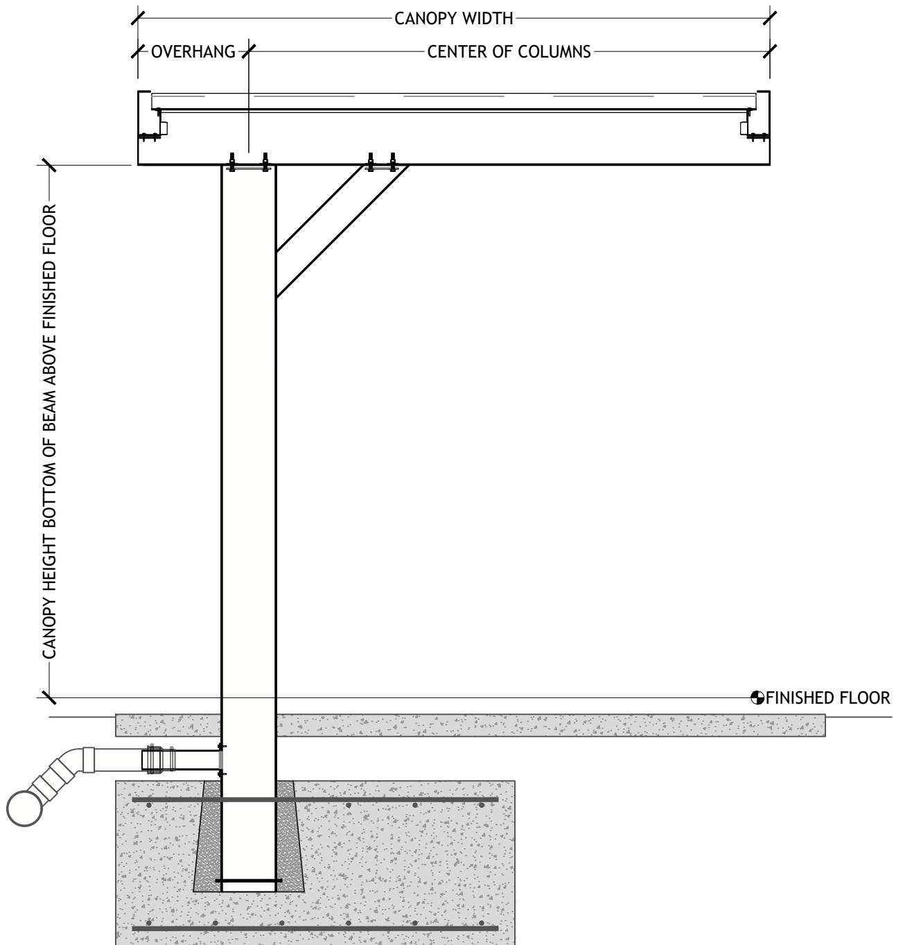
CANTILEVER BRACE SHORT SPAN FLUSH DECK UNDERGROUND DRAIN
