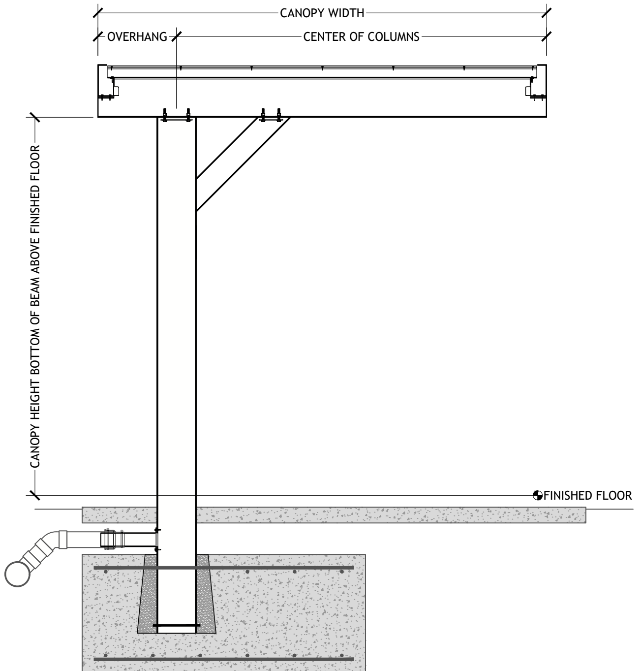
CANTILEVER BRACE SHORT SPAN PAN & CAP DECK UNDERGROUND DRAIN
