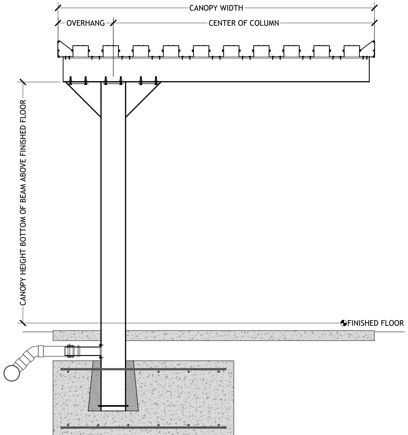
CANTILEVER GUSSET LONG SPAN HIGH PAN & CAP DECK UNDERGROUND DRAIN
