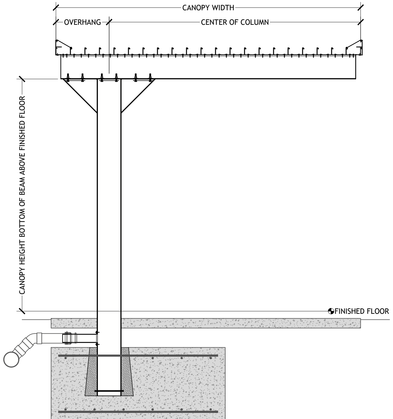
TWO POST LONG SPAN FLUSH DECK UNDERGROUND DRAIN
