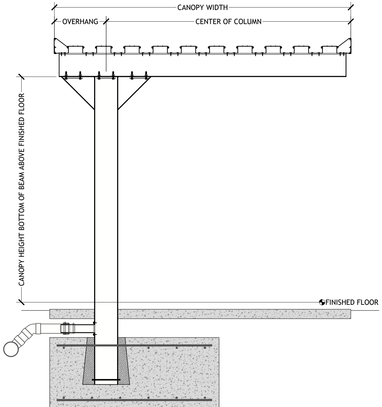
CANTILEVER GUSSET LONG SPAN PAN & CAP DECK UNDERGROUND DRAIN
