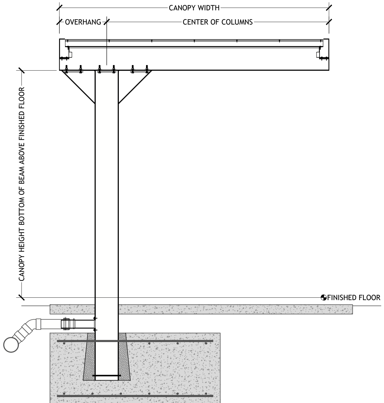
CANTILEVER GUSSET SHORT SPAN PAN & CAP DECK UNDERGROUND DRAIN
