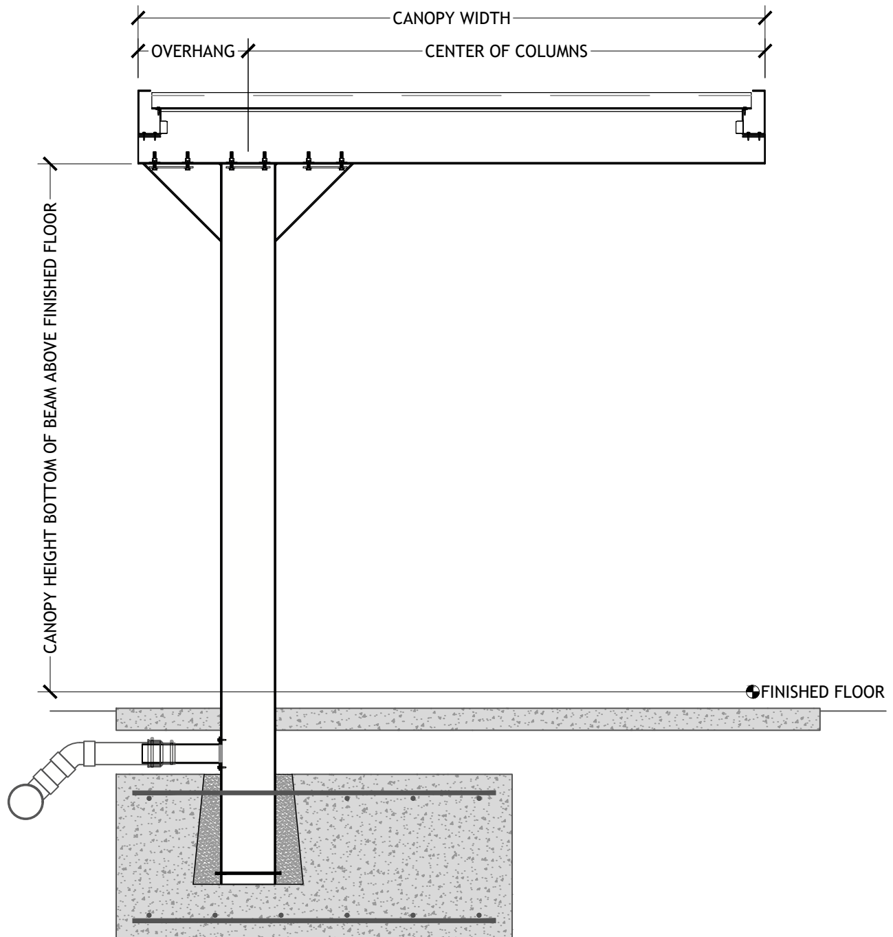
CANTILEVER GUSSET SHORT SPAN FLUSH DECK UNDERGROUND DRAIN
