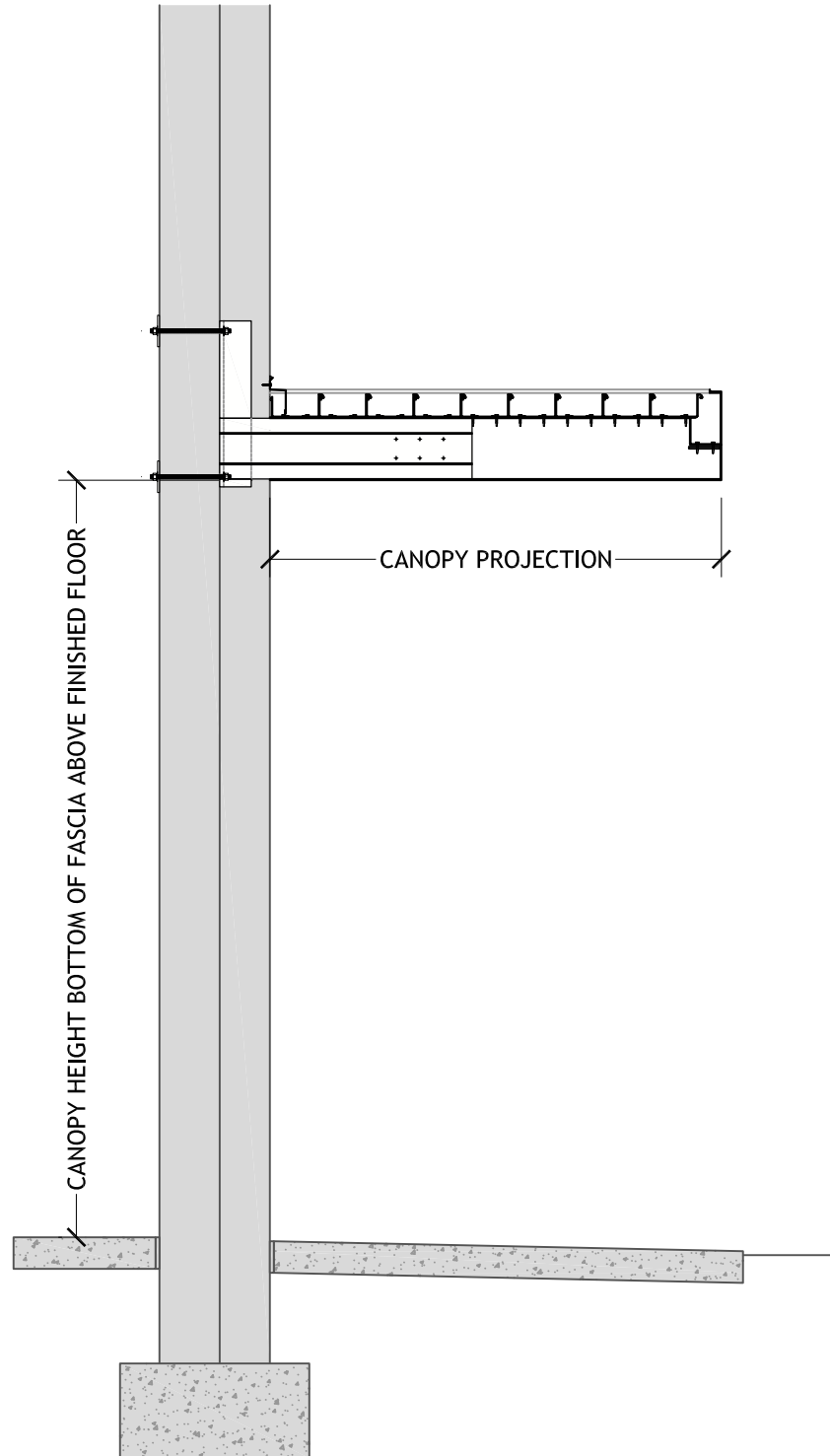
CAVITY WALL BOOT SUPPORT 7 INCH FASCIA GUTTER FLUSH DECK
