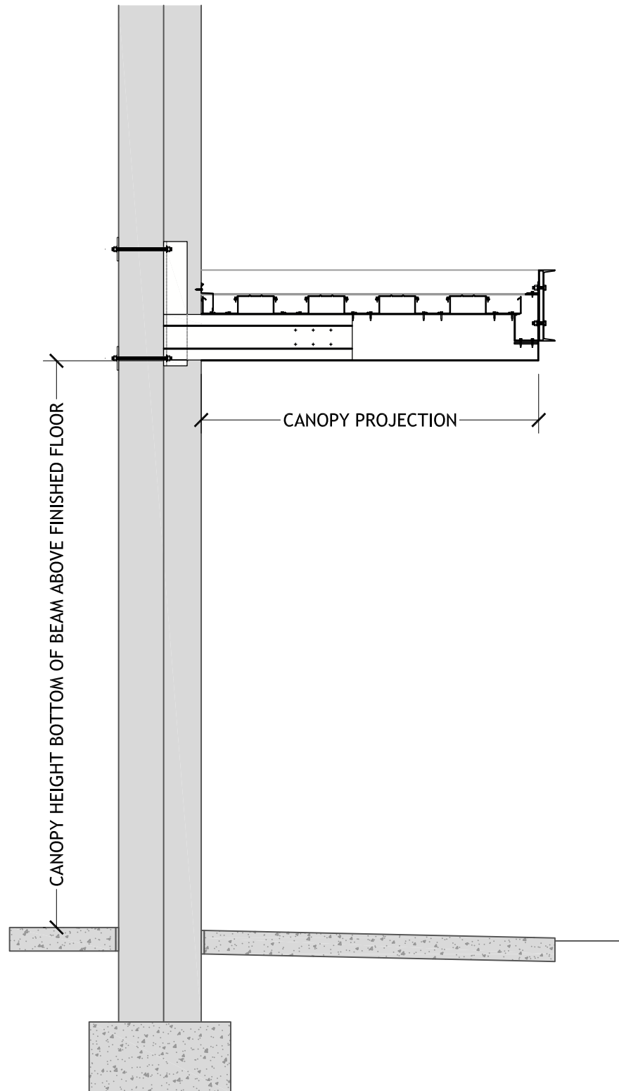
CAVITY WALL BOOT SUPPORT 8 INCH FASCIA GUTTER PAN AND CAP DECK BOLT ON HOLLOW BACK CHANNEL FASCIA
