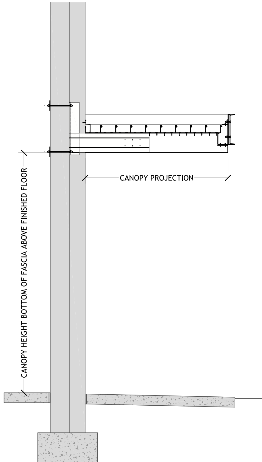
CAVITY WALL BOOT SUPPORT 8 INCH FASCIA GUTTER FLUSH DECK BOLT ON HOLLOW BACK CHANNEL FASCIA
