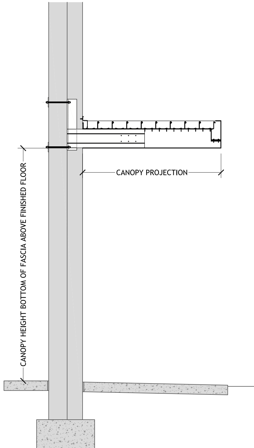
CAVITY WALL BOOT SUPPORT 8 INCH FASCIA GUTTER FLUSH DECK
