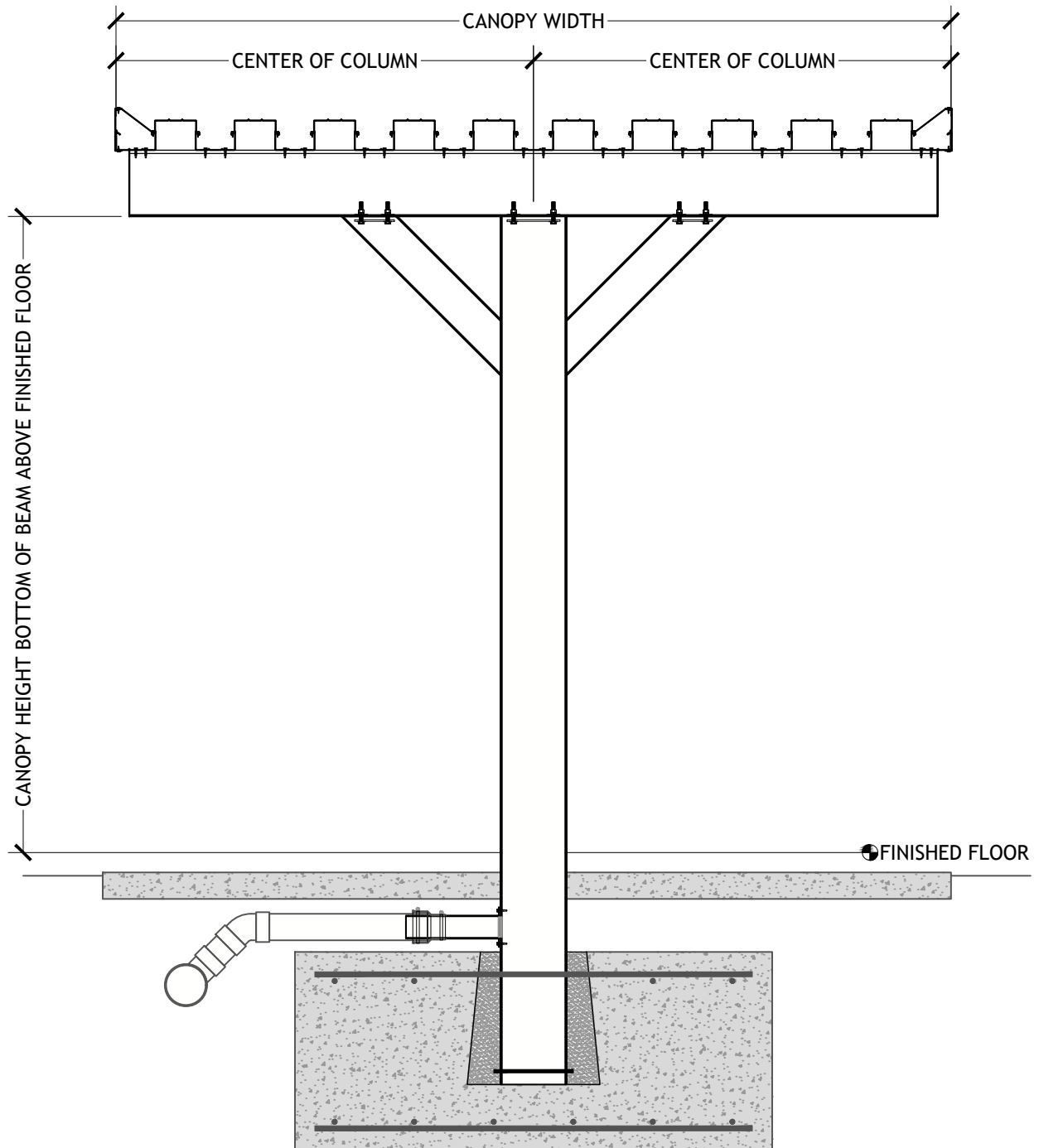
CENTER POST BRACE LONG SPAN HIGH PAN & CAP DECK UNDERGROUND DRAIN
