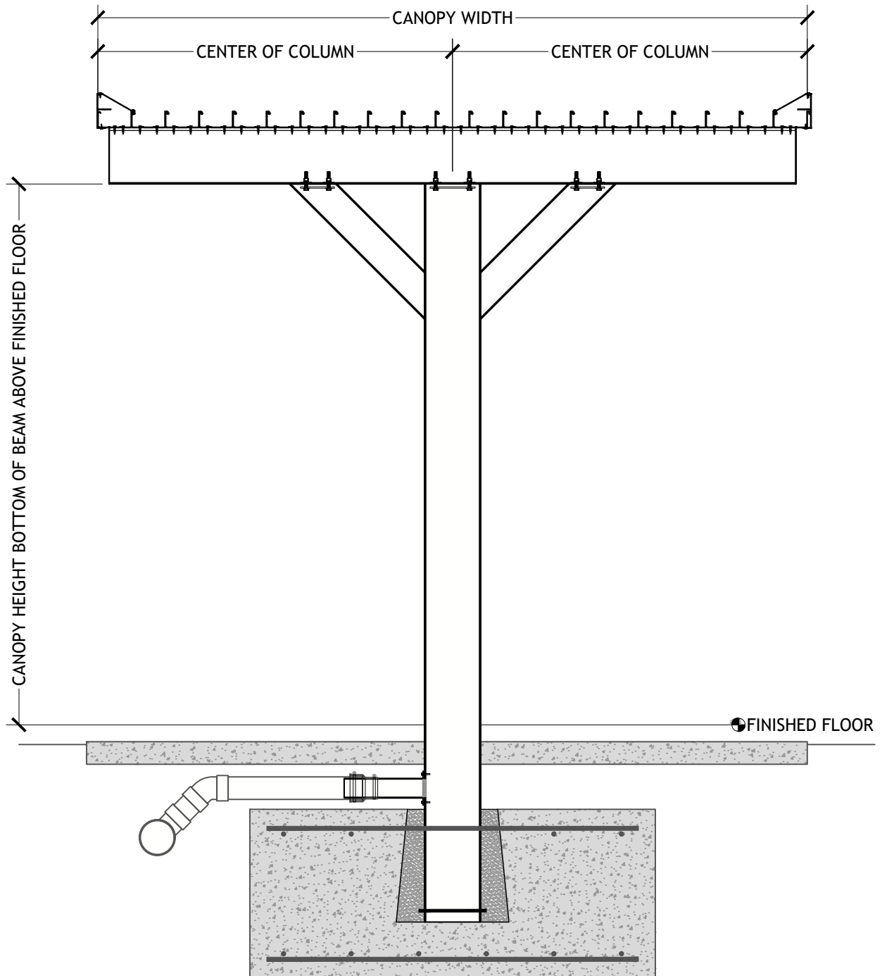
CENTER POST BRACE LONG SPAN FLUSH DECK UNDERGROUND DRAIN
