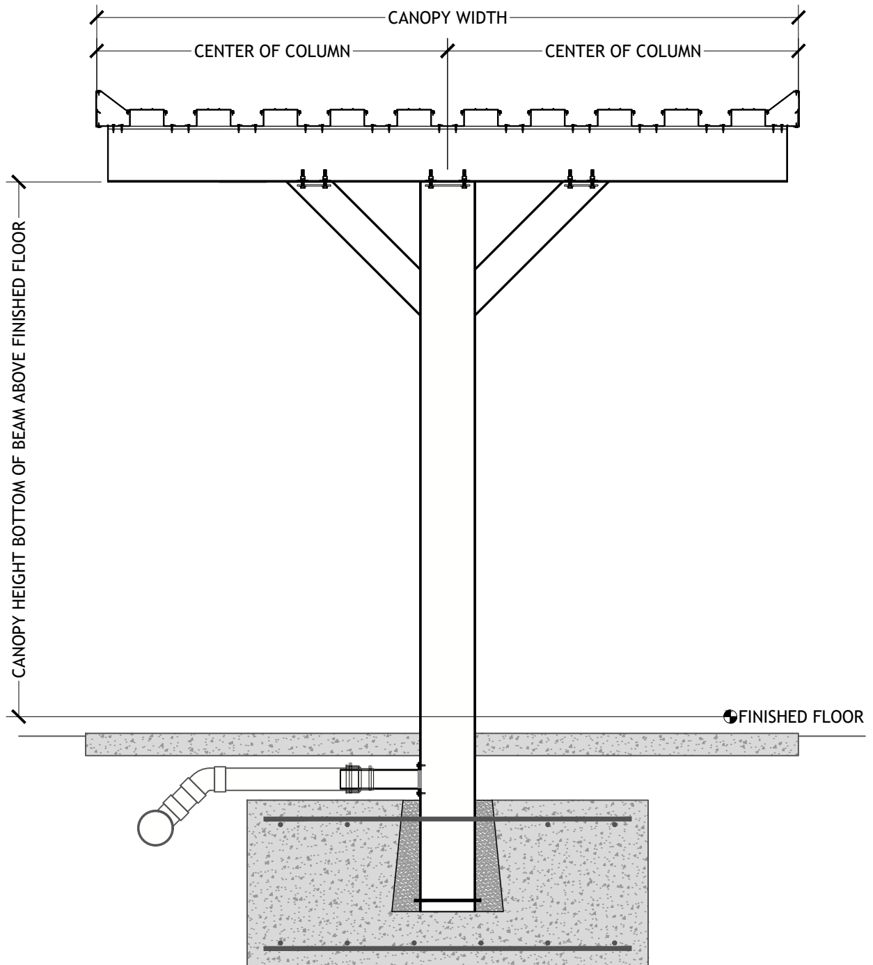
CENTER POST BRACE LONG SPAN PAN & CAP DECK UNDERGROUND DRAIN
