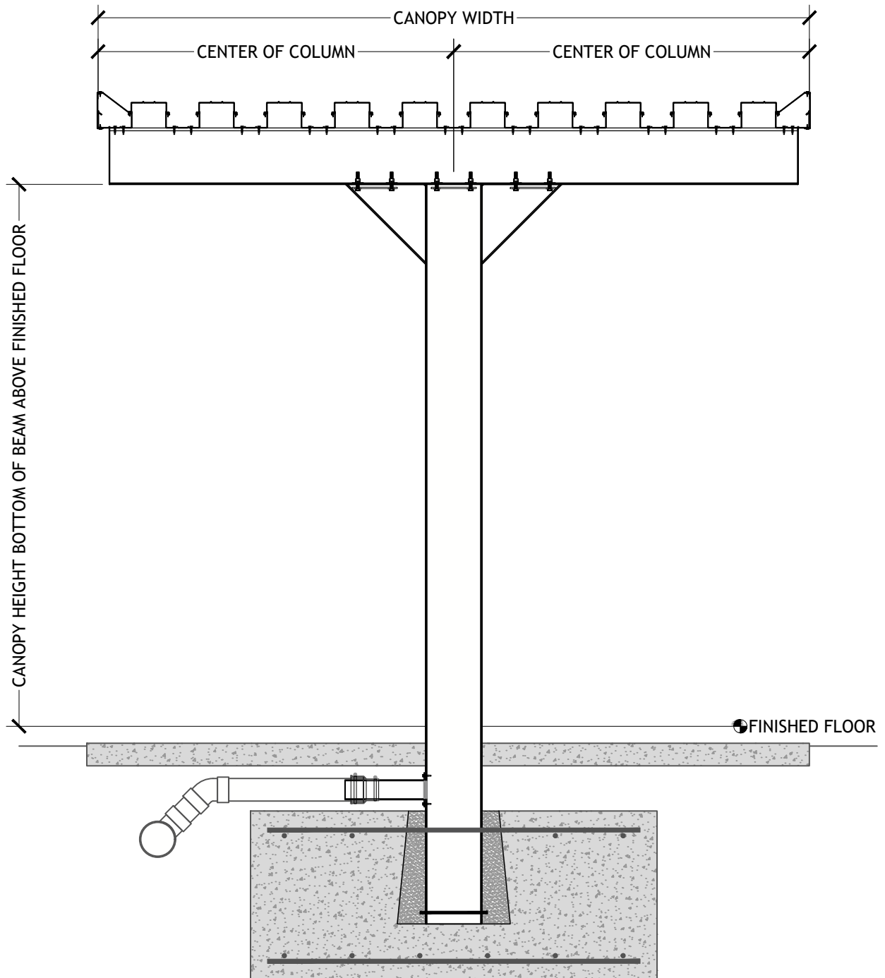
CENTER POST GUSSET LONG SPAN HIGH PAN & CAP DECK UNDERGROUND DRAIN
