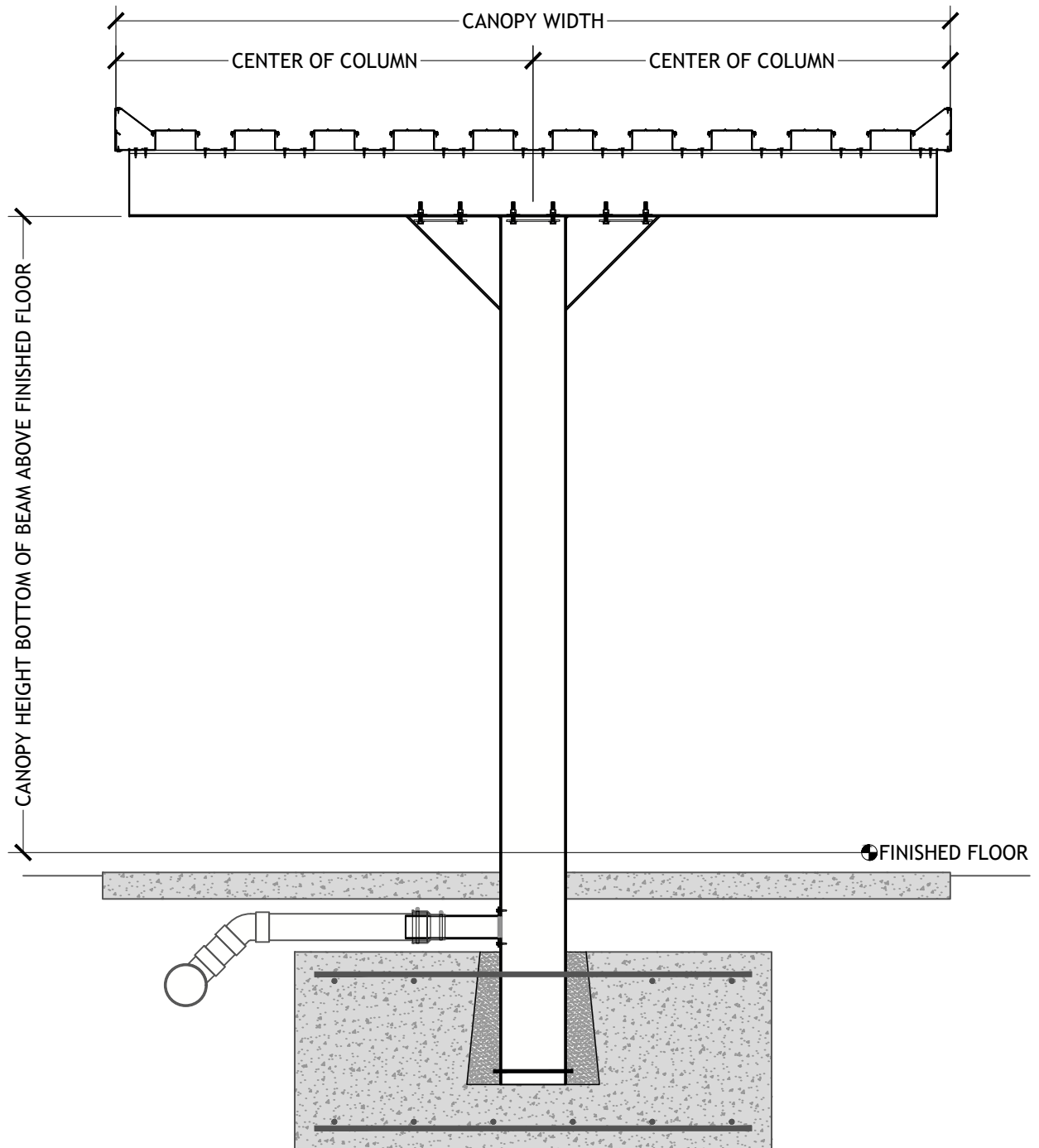
CENTER POST GUSSET LONG SPAN PAN & CAP DECK UNDERGROUND DRAIN
