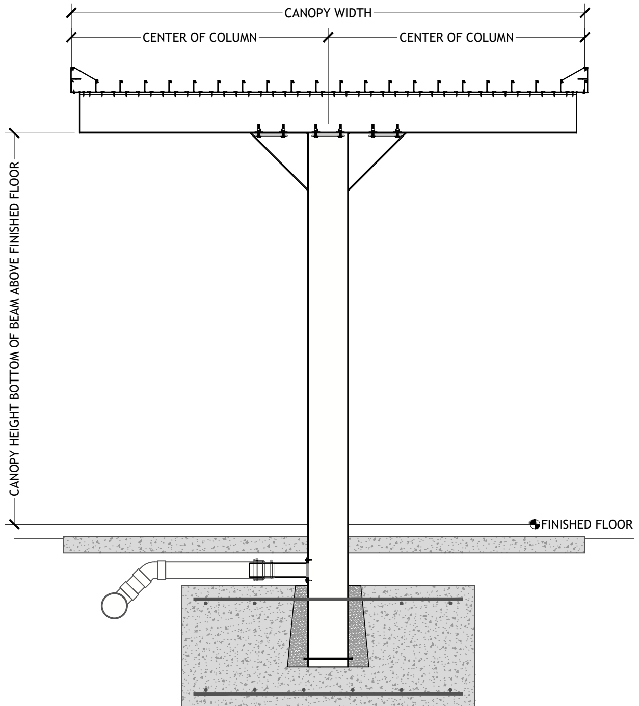
CENTER POST GUSSET LONG SPAN FLUSH DECK UNDERGROUND DRAIN
