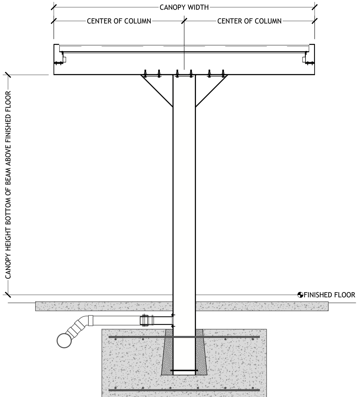
CENTER POST GUSSET SHORT SPAN FLUSH DECK UNDERGROUND DRAIN
