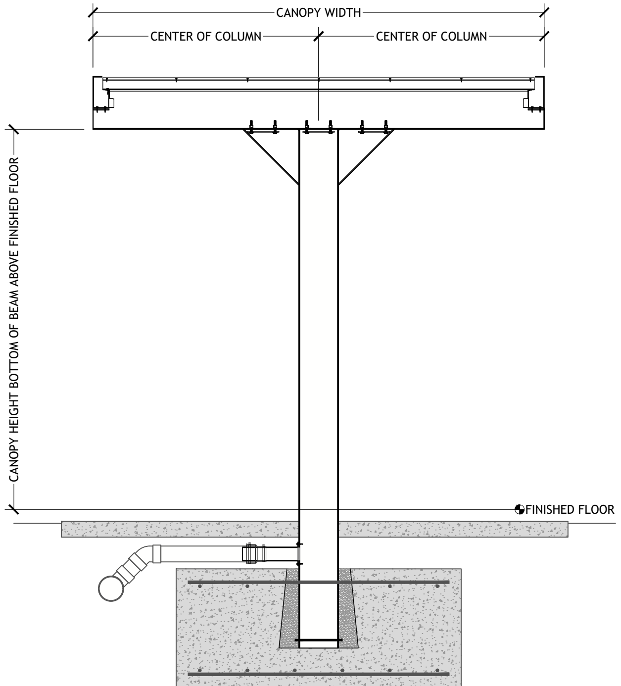
CENTER POST GUSSET SHORT SPAN PAN & CAP DECKING UNDERGROUND DRAIN
