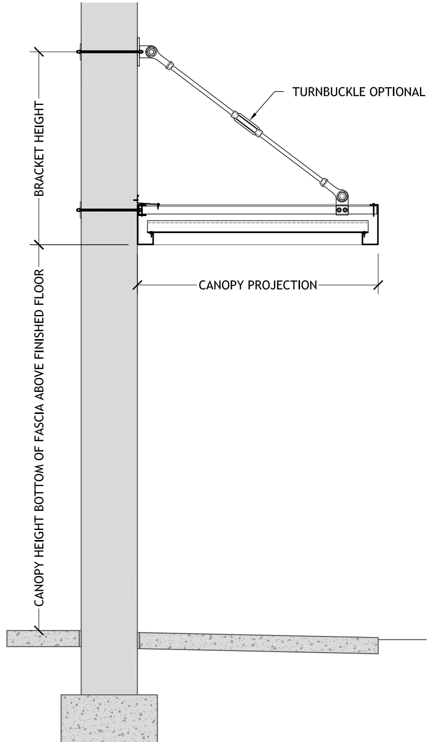
CLEVIS ARM OVERHEAD SUPPORT 10 INCH FASCIA GUTTER FLUSH DECK
