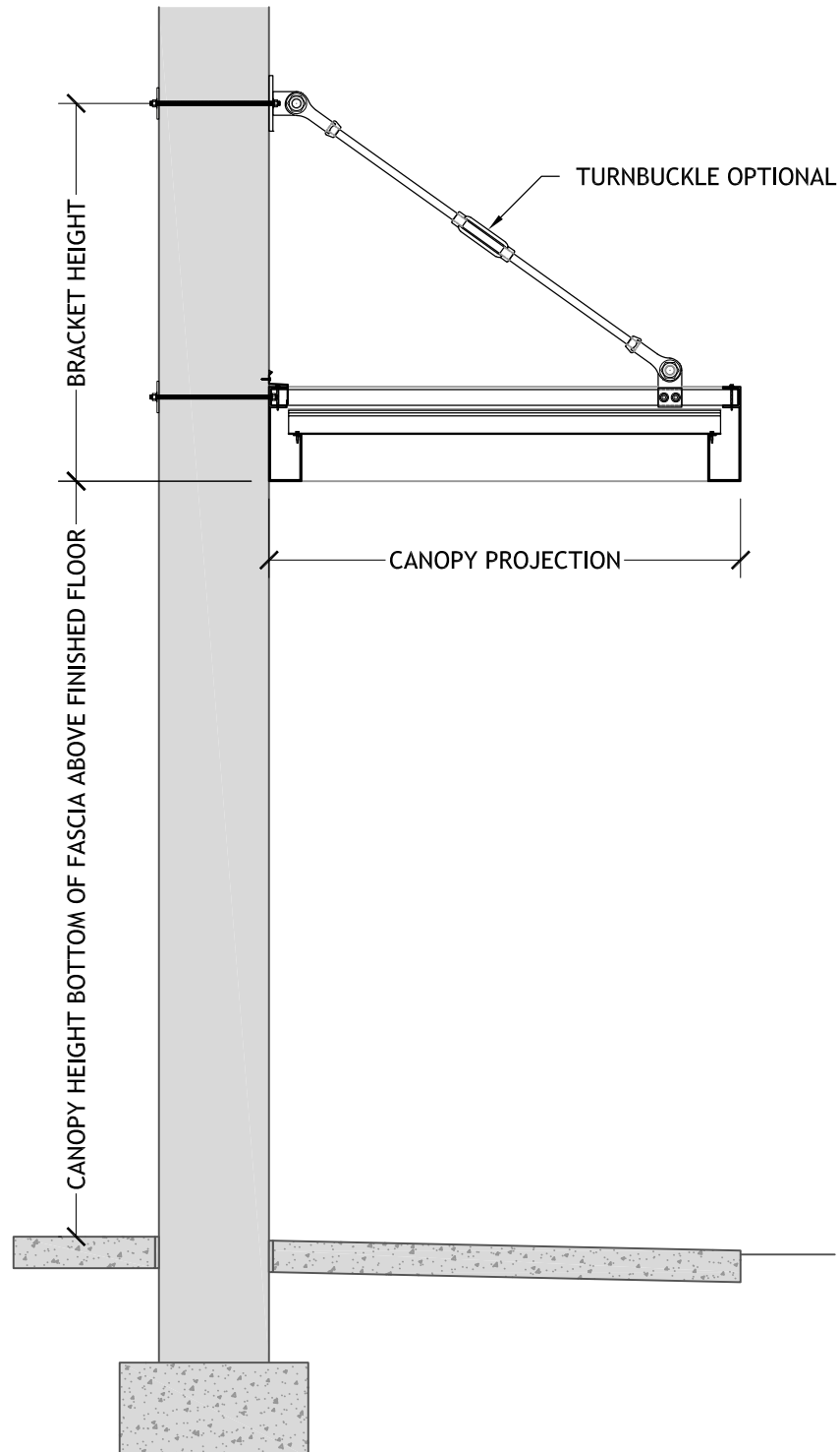
CLEVIS ARM OVERHEAD SUPPORT 12 INCH FASCIA GUTTER PAN AND CAP DECK
