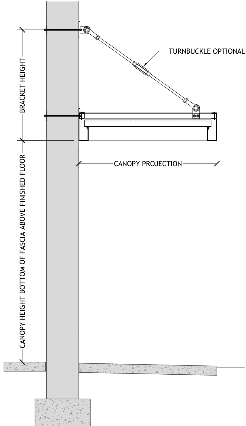
CLEVIS ARM OVERHEAD SUPPORT 12 INCH FASCIA GUTTER FLUSH DECK
