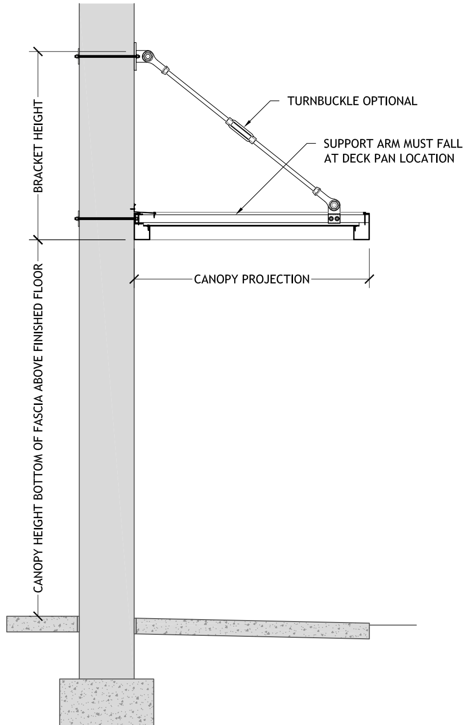
CLEVIS ARM OVERHEAD SUPPORT 7 INCH FASCIA GUTTER FLUSH DECK
