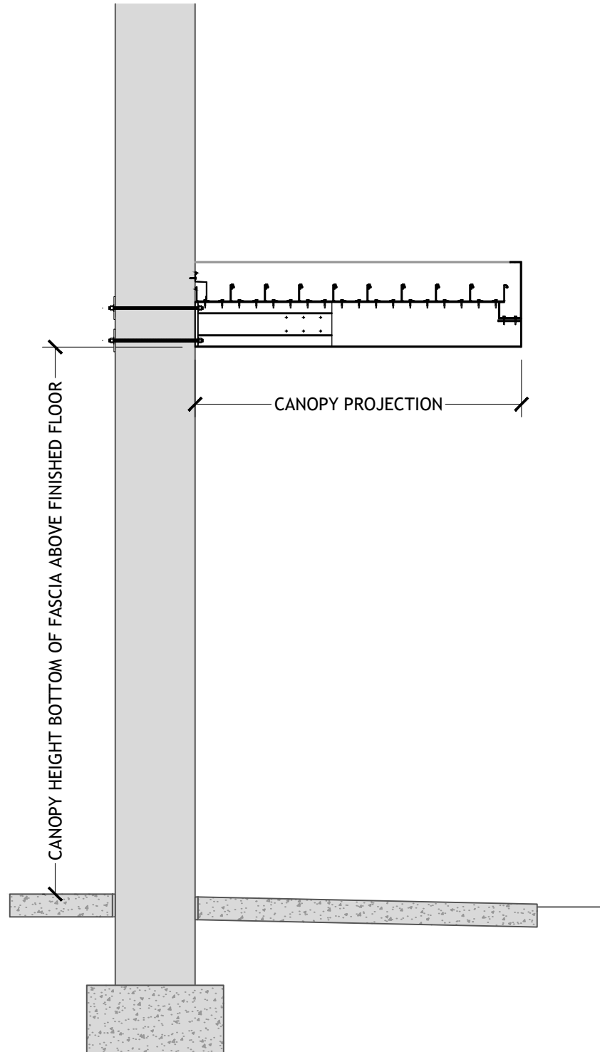
FACE MOUNT BOOT SUPPORT 10 INCH FASCIA GUTTER FLUSH DECK
