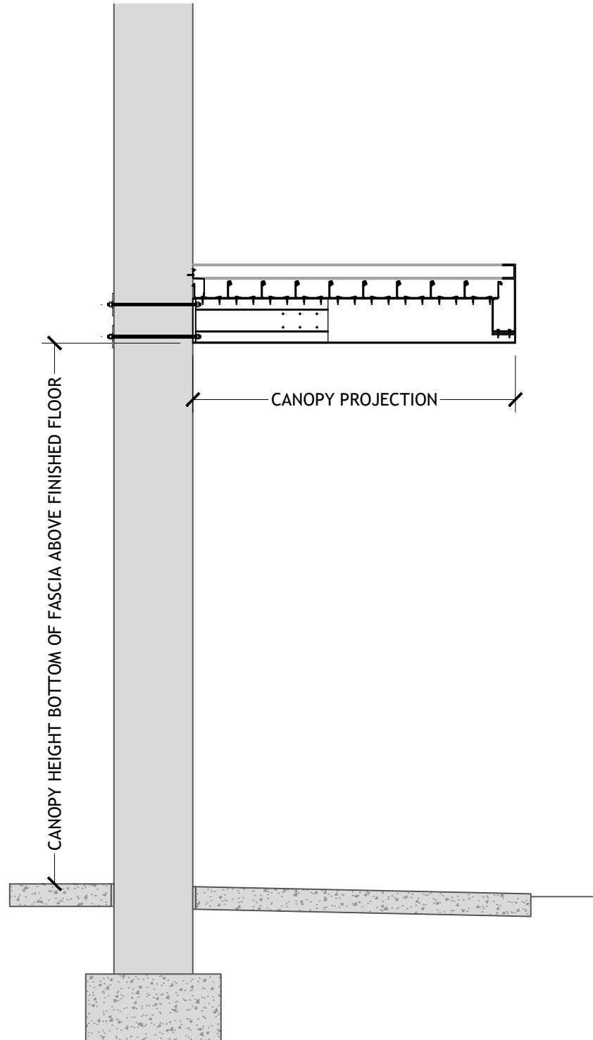
FACE MOUNT BOOT SUPPORT 12 INCH FASCIA GUTTER FLUSH DECK
