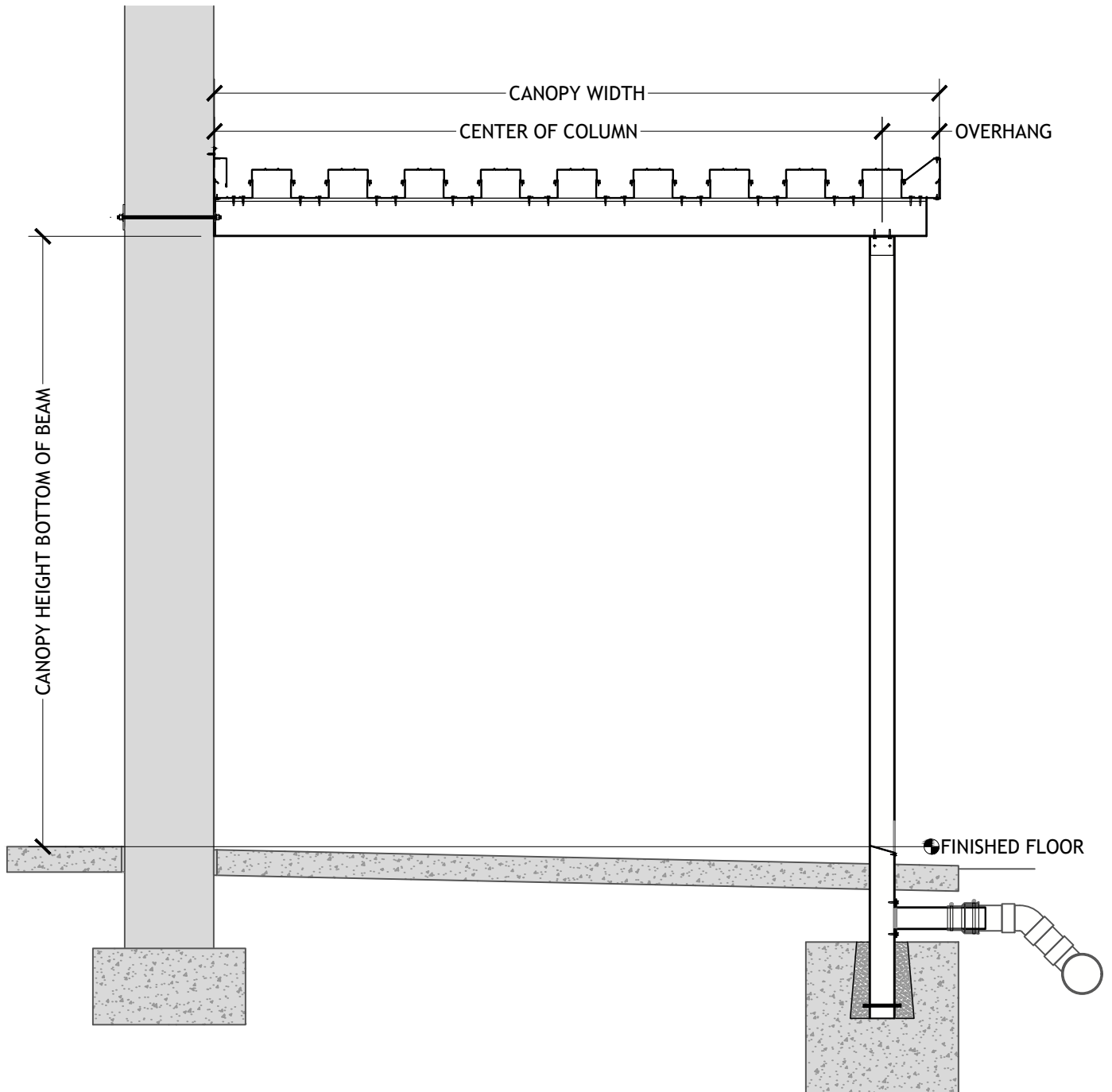
LEAN-TO LONG SPAN HIGH PAN & CAP DECK UNDERGROUND DRAIN
