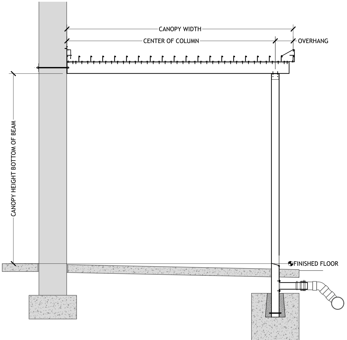
LEAN-TO LONG SPAN FLUSH DECK UNDERGROUND DRAIN
