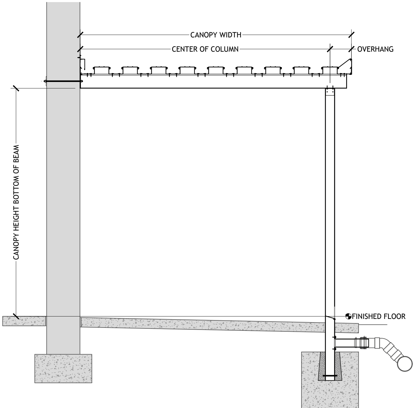
LEAN-TO LONG SPAN PAN & CAP DECK UNDERGROUND DRAIN
