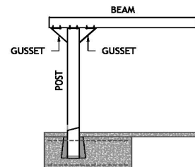
CANTILEVER GUSSET SYSTEM
