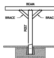
CENTER POST BRACE SYSTEM
