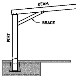
PITCHED CANTILEVER GUSSET SYSTEM
