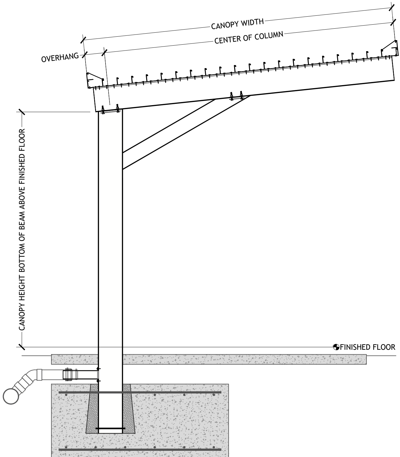
PITCHED CANTILEVER BRACE LONG SPAN FLUSH DECK UNDERGROUND DRAIN
