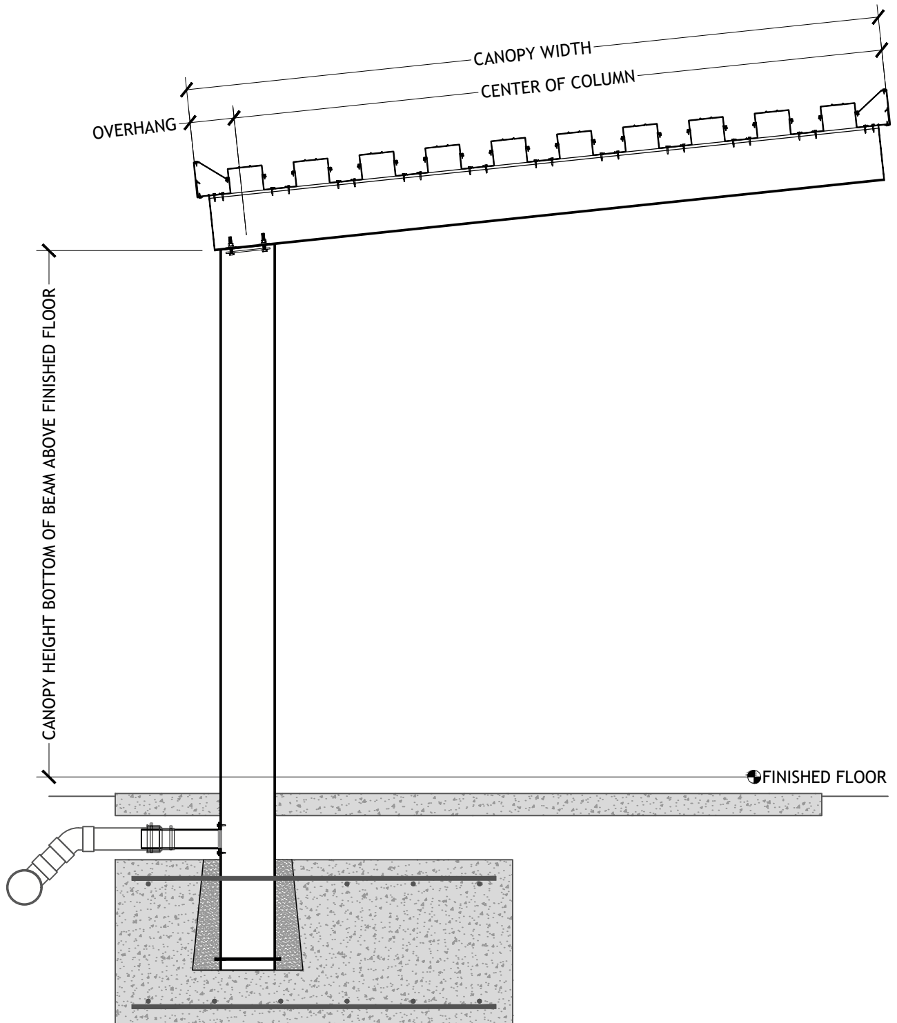
PITCHED CANTILEVER BRACE LONG SPAN HIGH PAN & CAP DECK UNDERGROUND DRAIN
