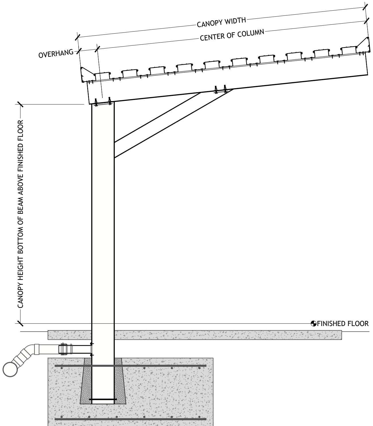
PITCHED CANTILEVER BRACE LONG SPAN PAN & CAP DECK UNDERGROUND DRAIN
