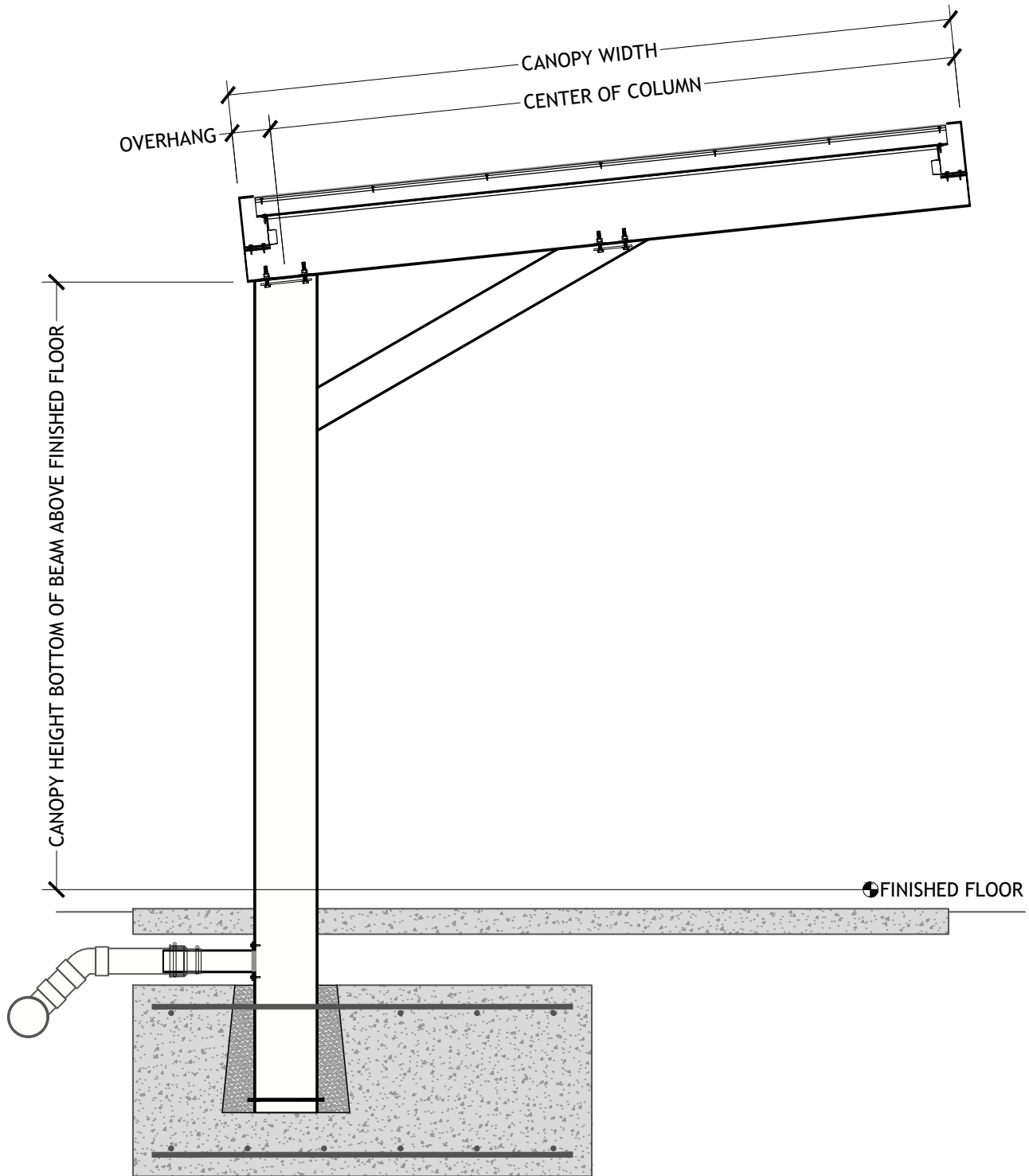
PITCHED CANTILEVER BRACE SHORT SPAN PAN & CAP DECKING UNDERGROUND DRAIN
