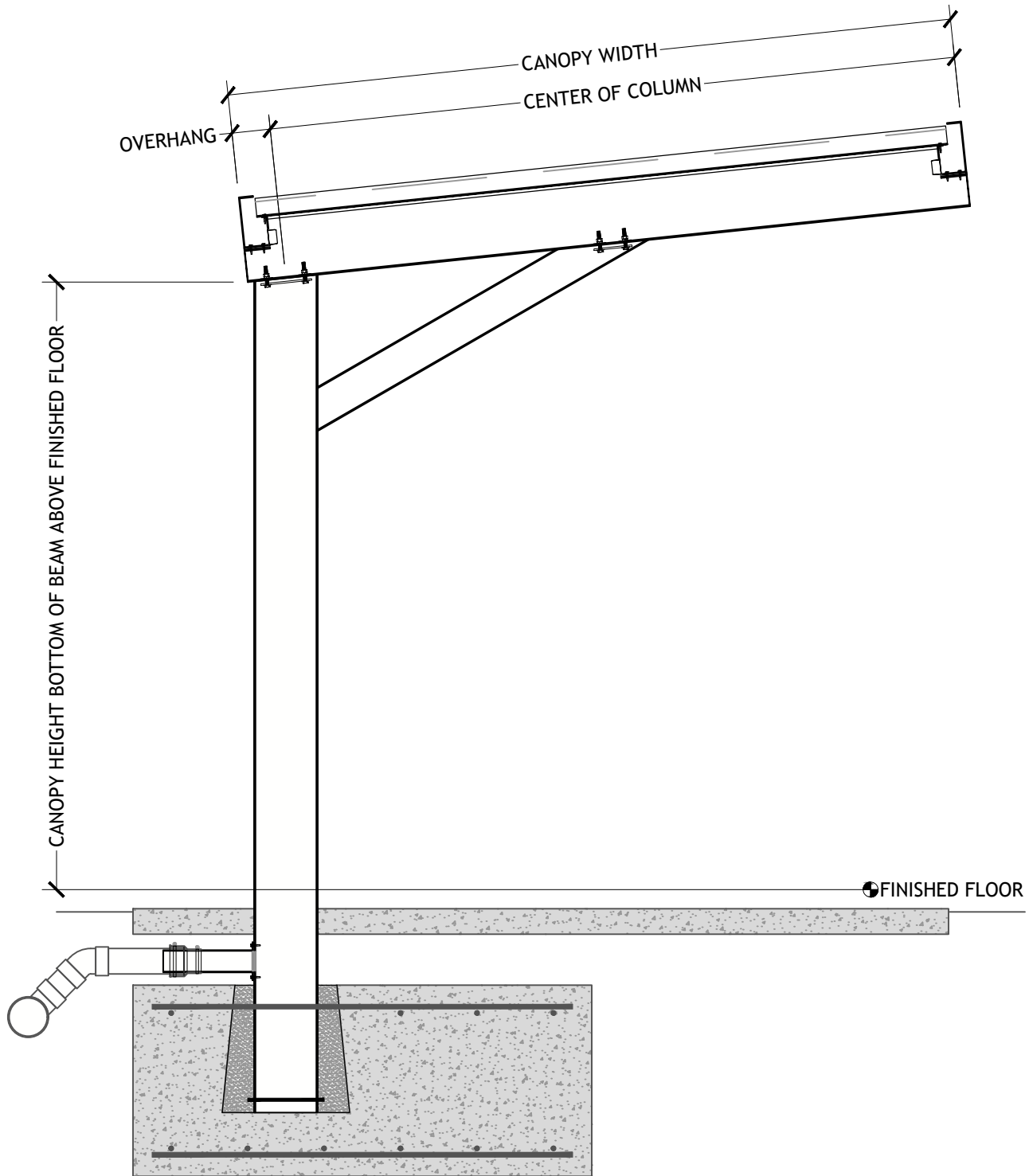
PITCHED CANTILEVER BRACE SHORT SPAN FLUSH DECK UNDERGROUND DRAIN
