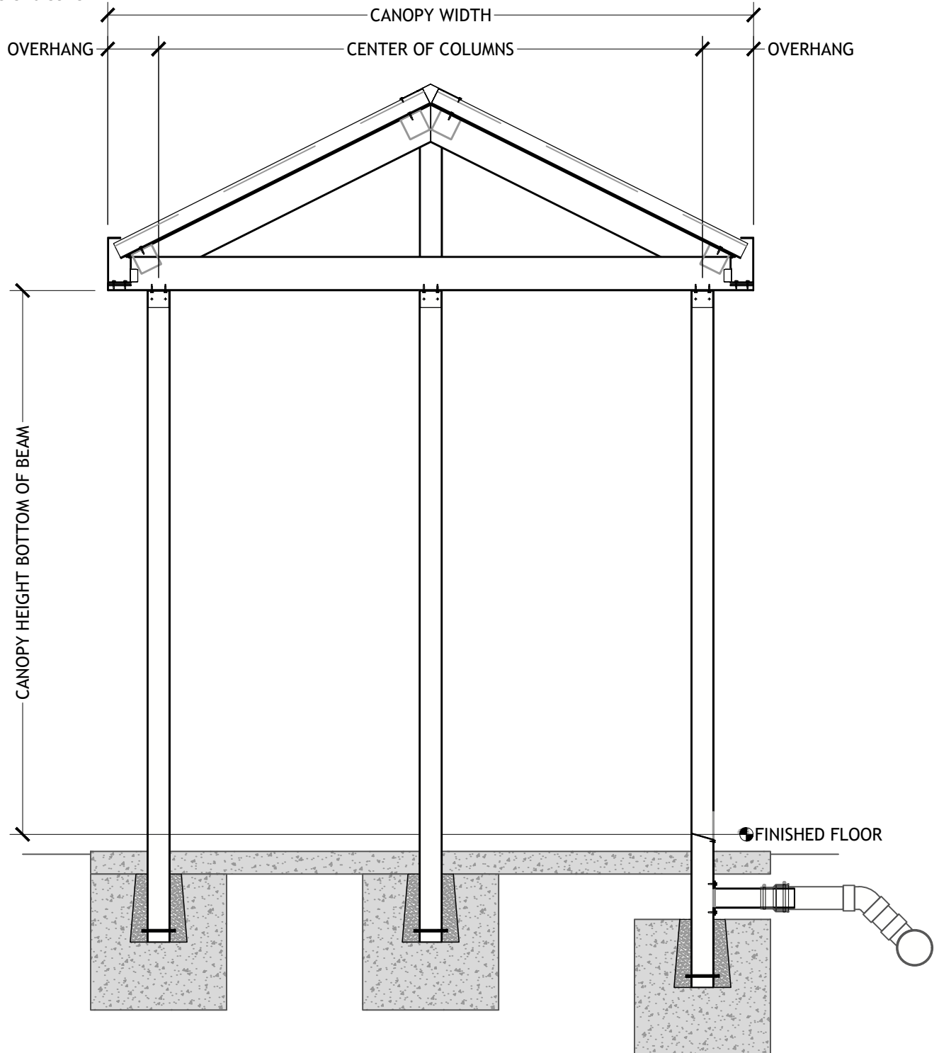
PITCHED TRUSS THREE POST FLUSH DECK UNDERGROUND DRAIN
