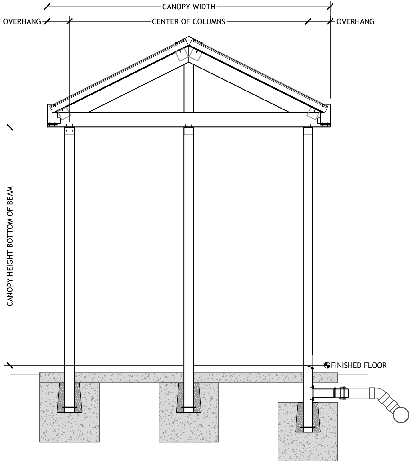
PITCHED TRUSS THREE POST PAN & CAP DECK UNDERGROUND DRAIN
