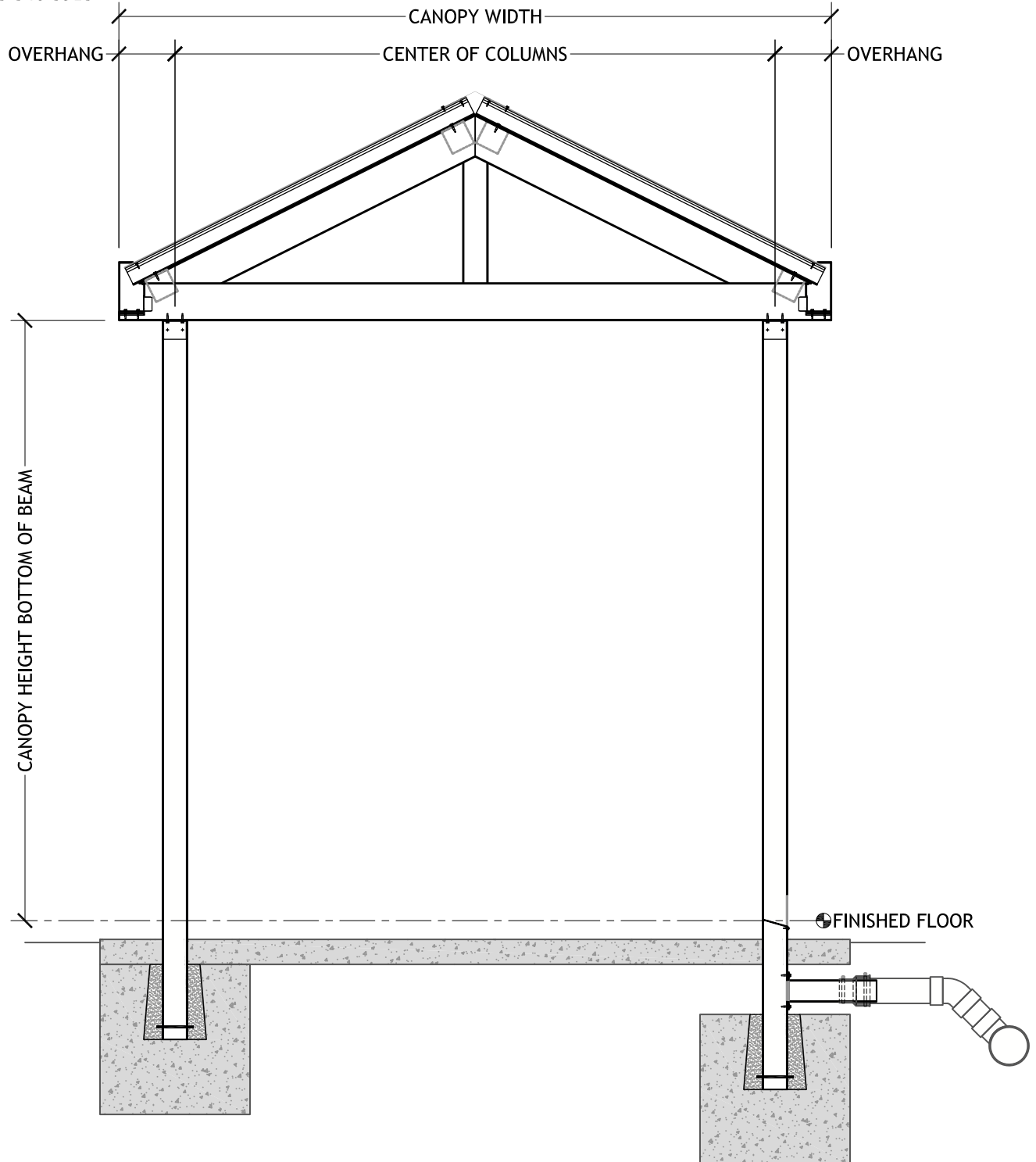
PITCHED TRUSS PAN & CAP DECK UNDERGROUND DRAIN
