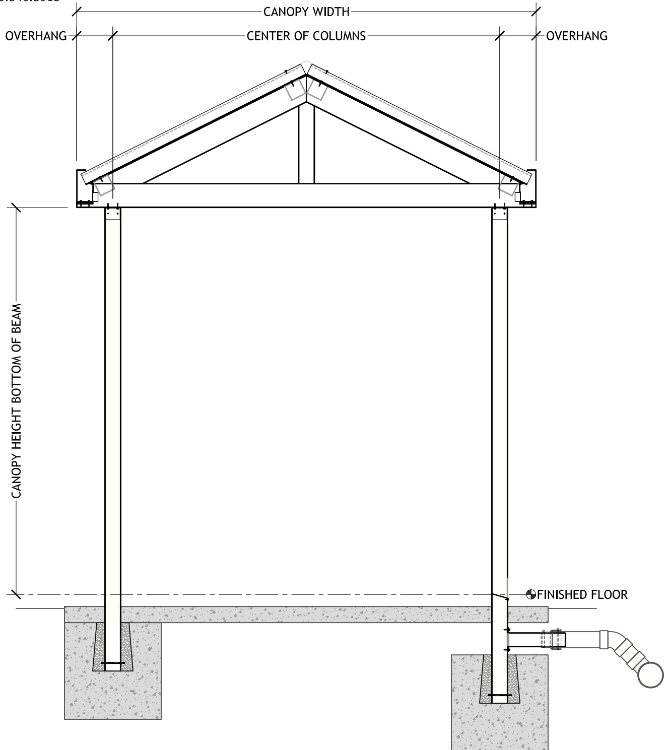
PITCHED TRUSS FLUSH DECK UNDERGROUND DRAIN
