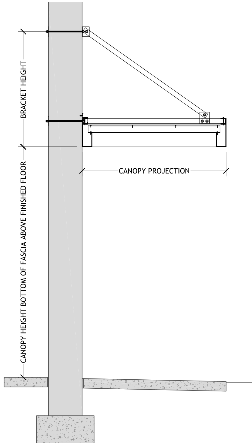
STANDARD OVERHEAD SUPPORT 12 INCH FASCIA GUTTER PAN AND CAP DECK
