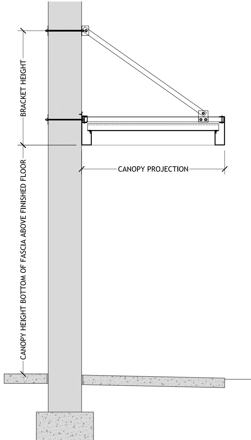
STANDARD OVERHEAD SUPPORT 12 INCH FASCIA GUTTER FLUSH DECK
