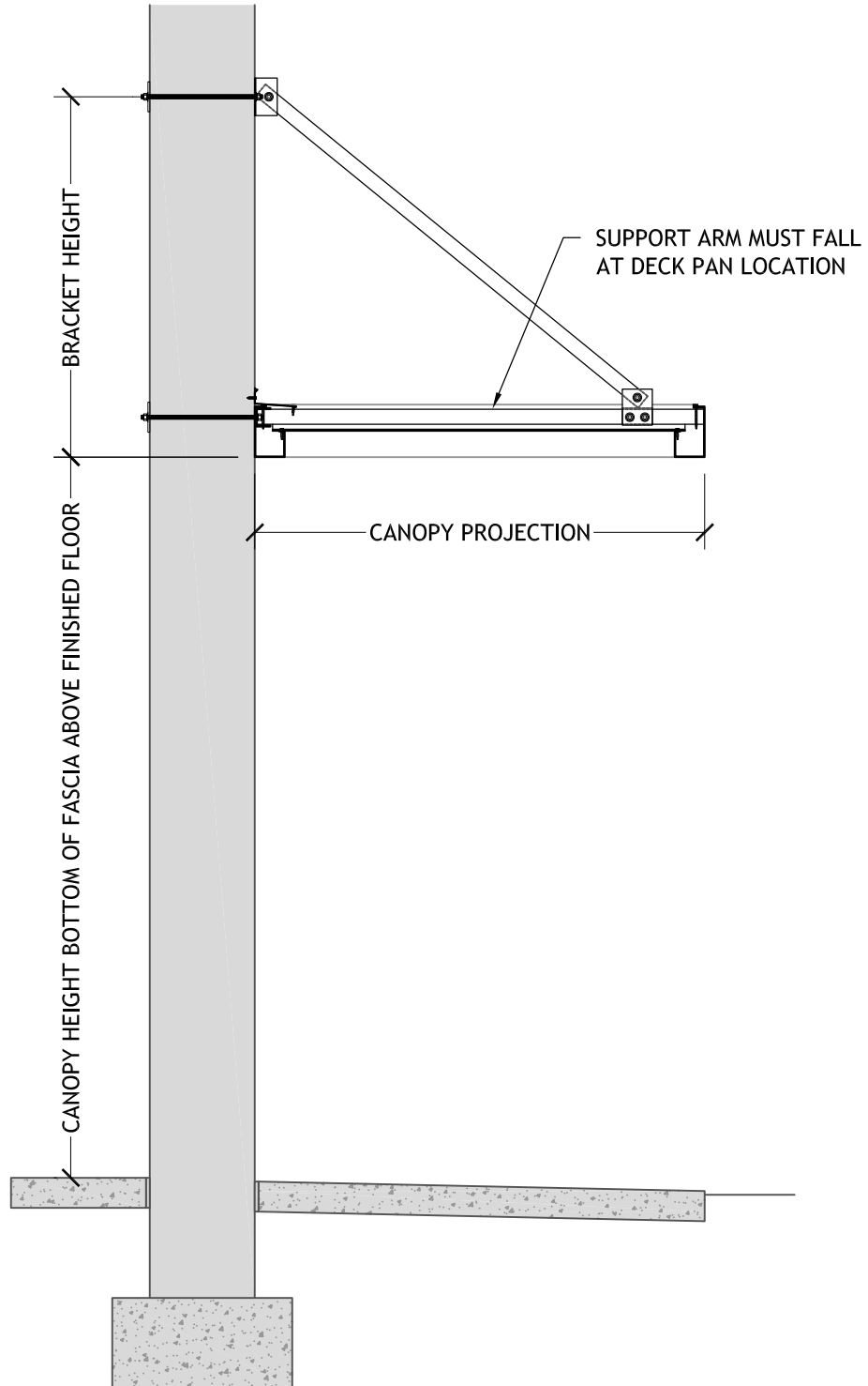
STANDARD OVERHEAD SUPPORT 7 INCH FASCIA GUTTER FLUSH DECK
