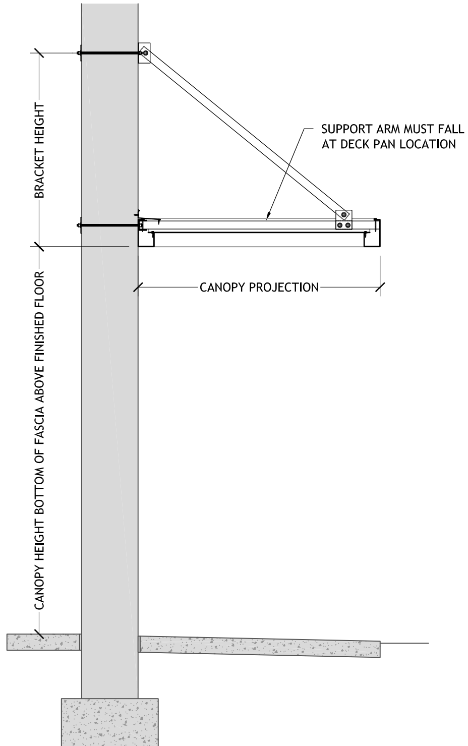
STANDARD OVERHEAD SUPPORT 7 INCH FASCIA GUTTER PAN AND CAP DECK
