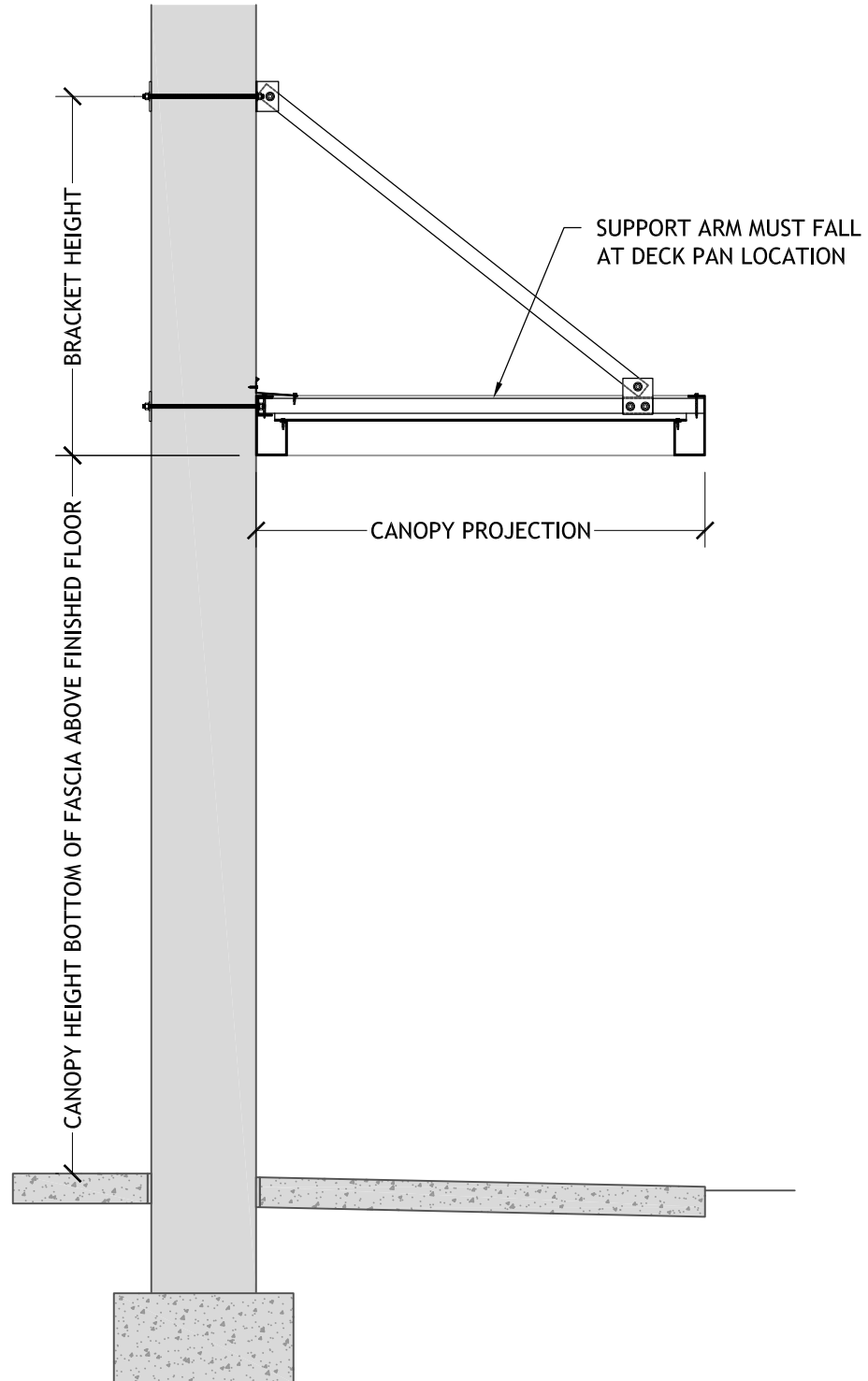
STANDARD OVERHEAD SUPPORT 8 INCH FASCIA GUTTER FLUSH DECK
