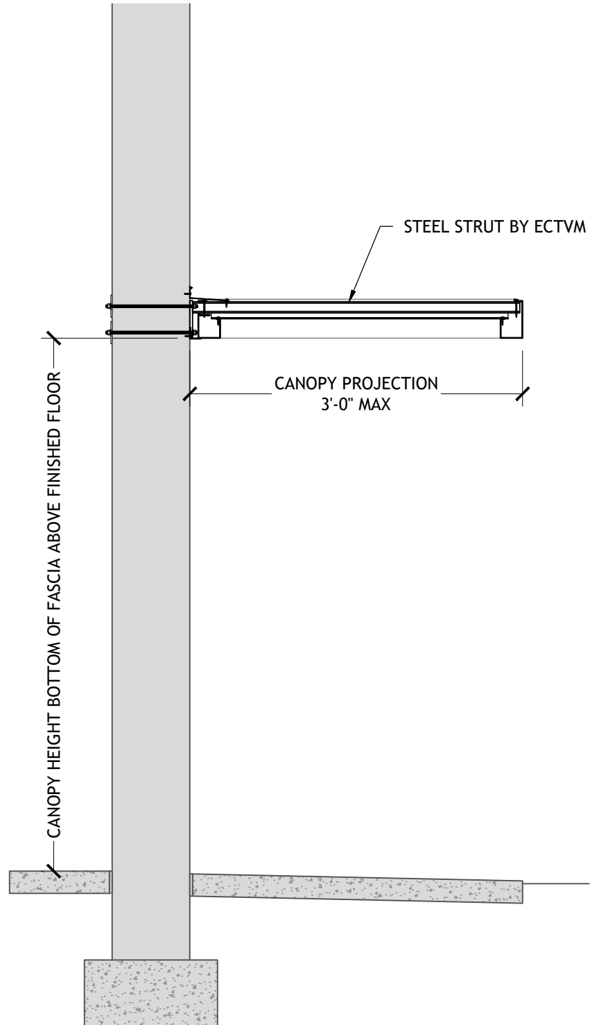
STRUT SUPPORT 7 INCH FASCIA FLUSH DECK
