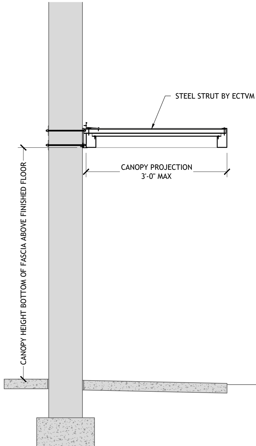
STRUT SUPPORT 8 INCH FASCIA FLUSH DECK
