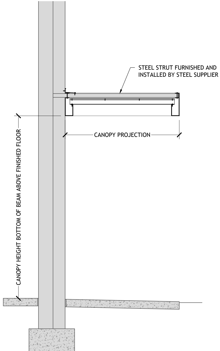
STRUT SUPPORT 12 INCH FASCIA PAN AND CAP DECK
