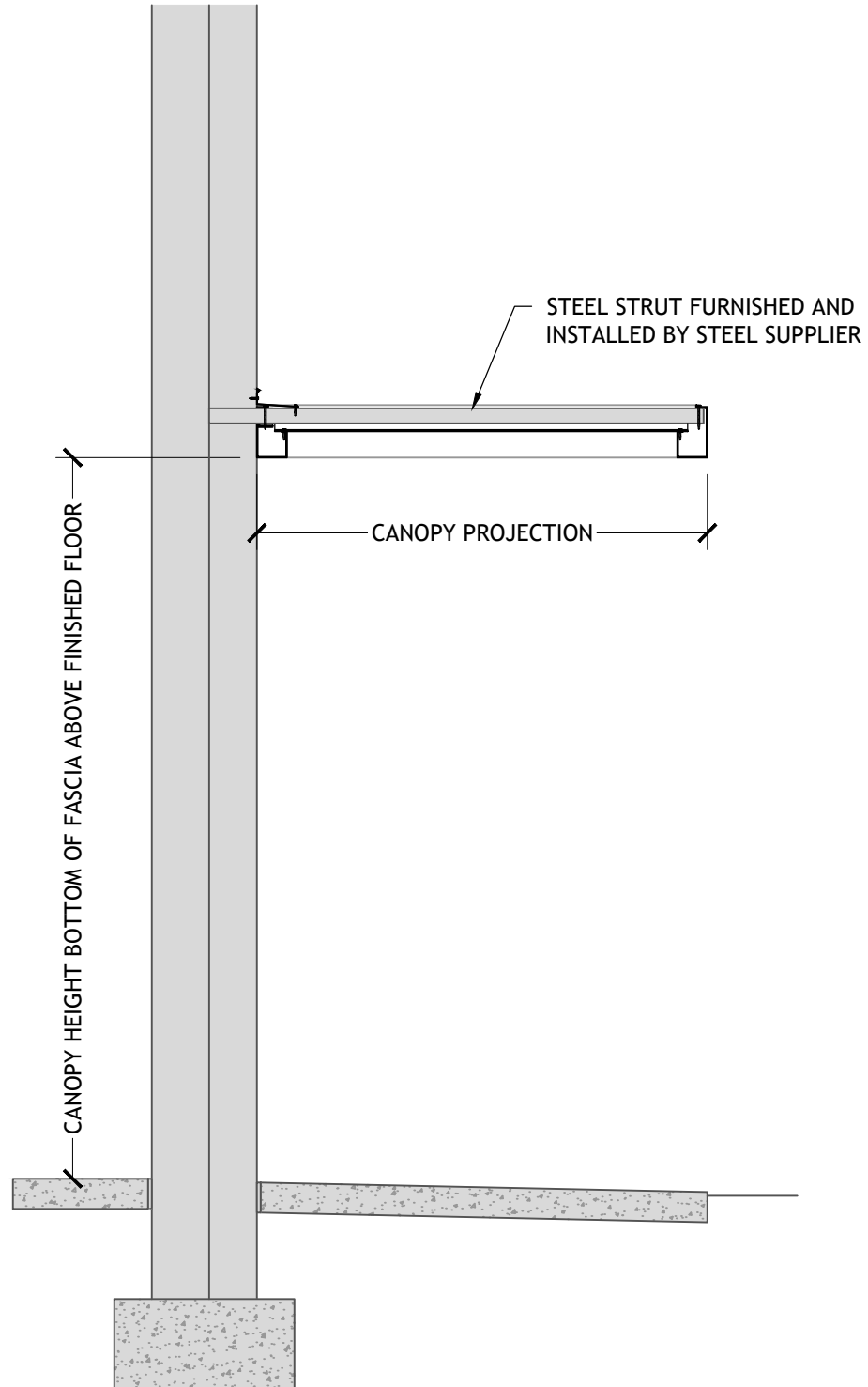
STRUT SUPPORT 7 INCH FASCIA FLUSH DECK
