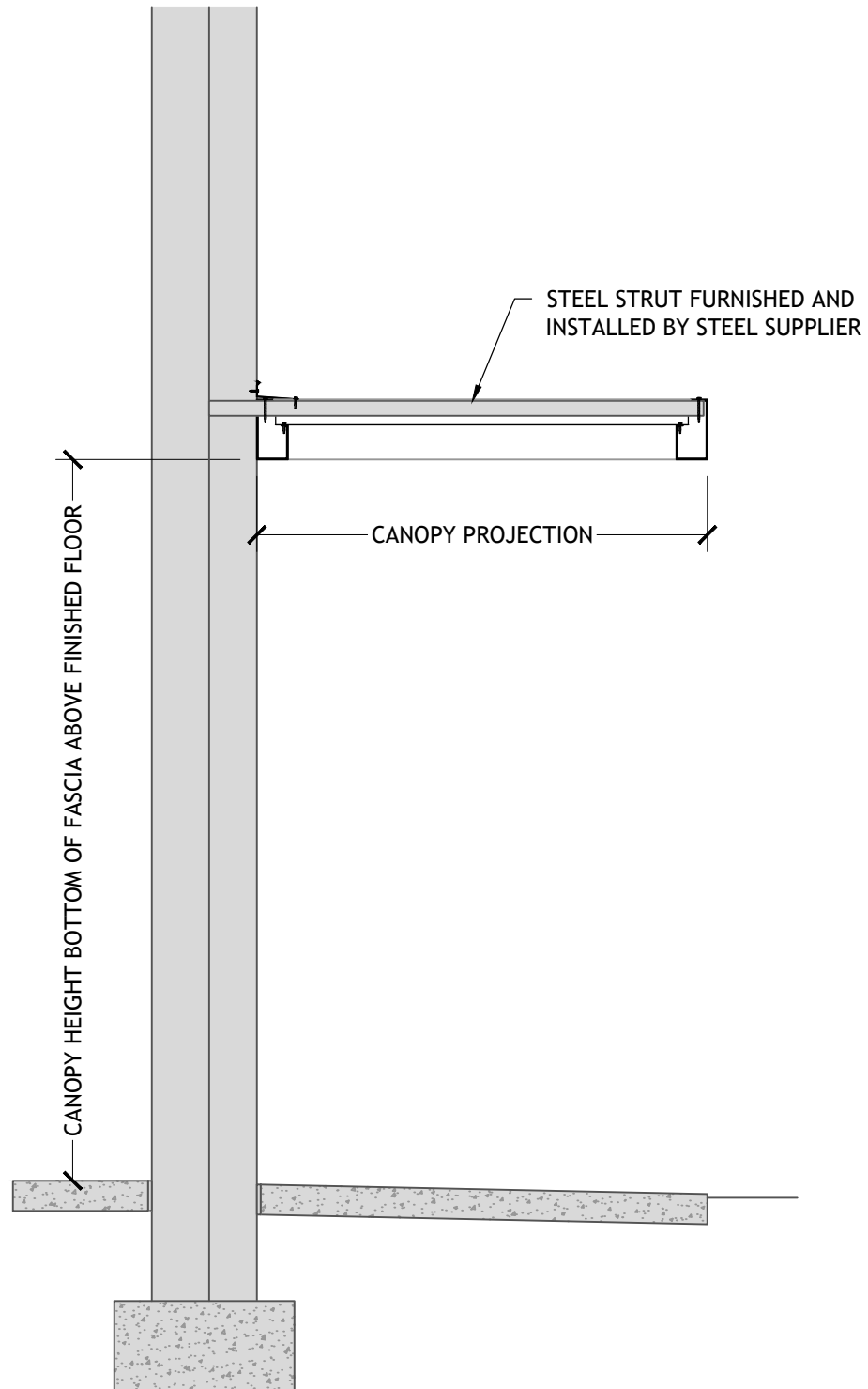
STRUT SUPPORT 8 INCH FASCIA PAN AND CAP DECK
