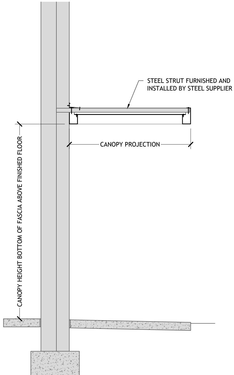
STRUT SUPPORT 8 INCH FASCIA FLUSH DECK
