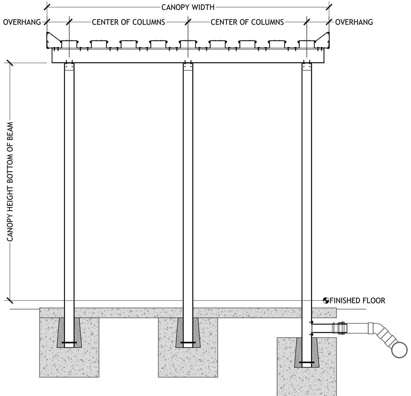
THREE POST LONG SPAN PAN & CAP DECK UNDERGROUND DRAIN
