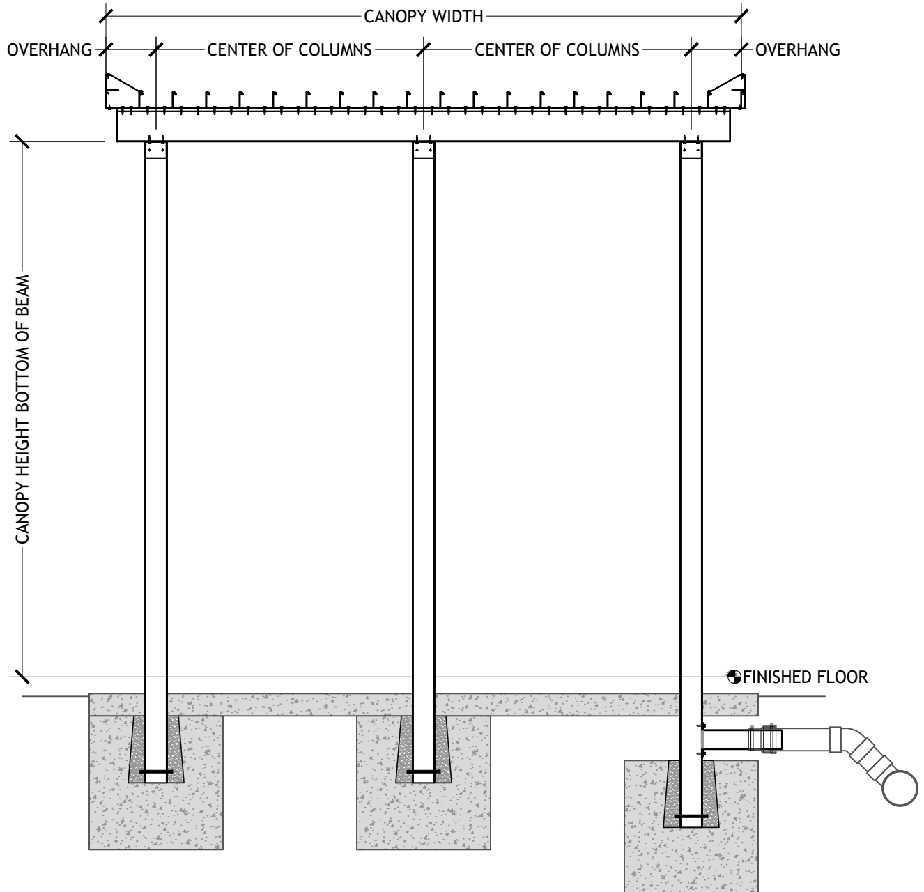
THREE POST LONG SPAN FLUSH DECK UNDERGROUND DRAIN
