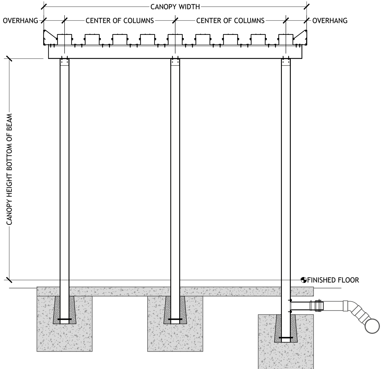
THREE POST LONG SPAN HIGH PAN & CAP DECK UNDERGROUND DRAIN
