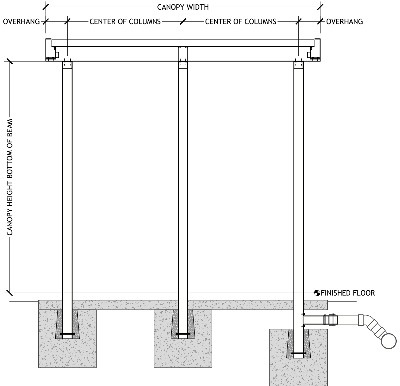
THREE POST SHORT SPAN FLUSH DECK UNDERGROUND DRAIN
