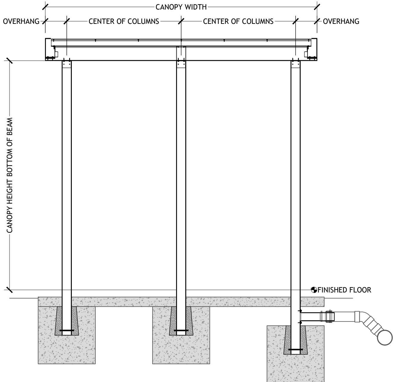
THREE POST SHORT SPAN PAN & CAP DECK UNDERGROUND DRAIN
