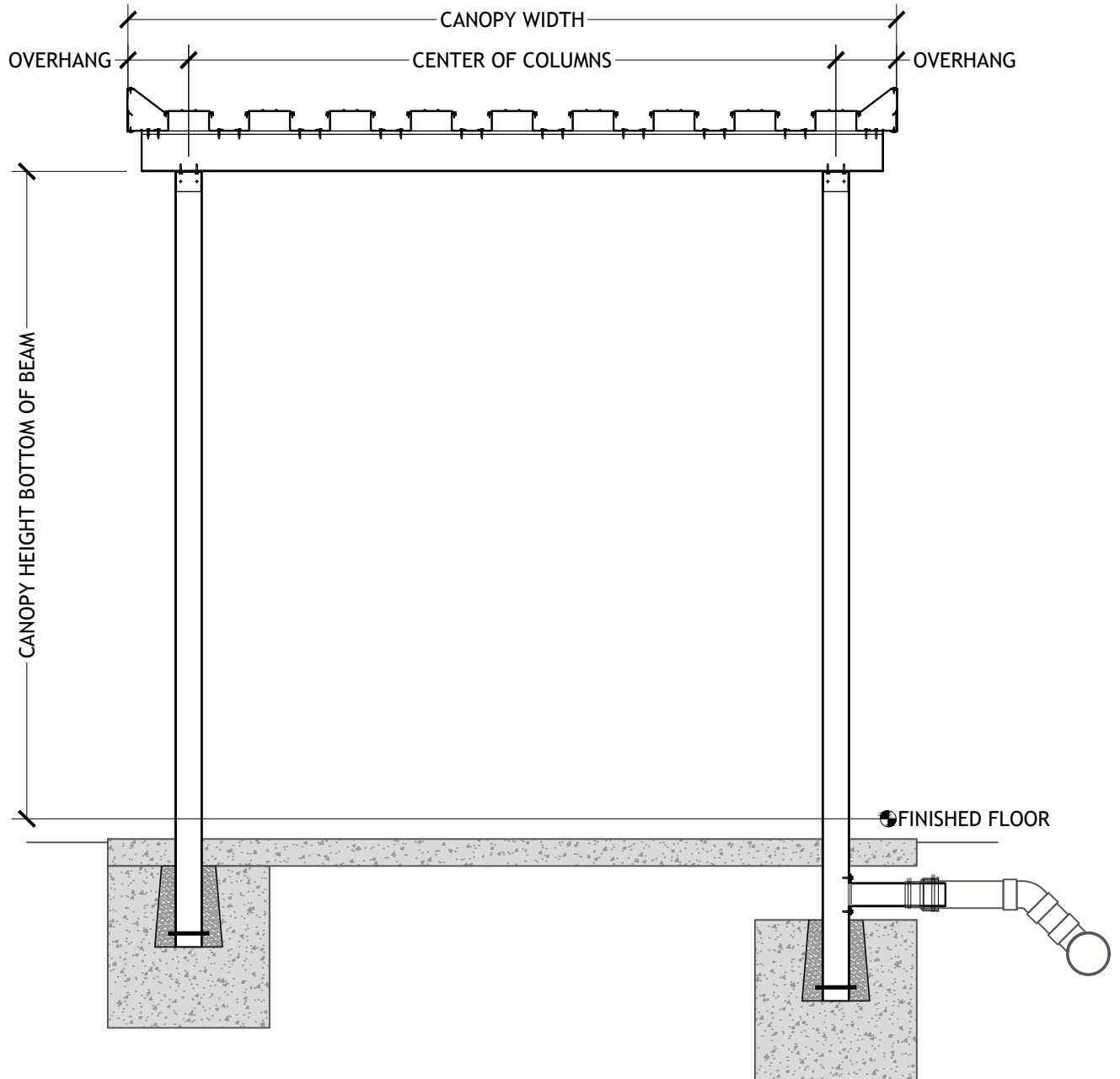
TWO POST LONG SPAN PAN & CAP DECK UNDERGROUND DRAIN
