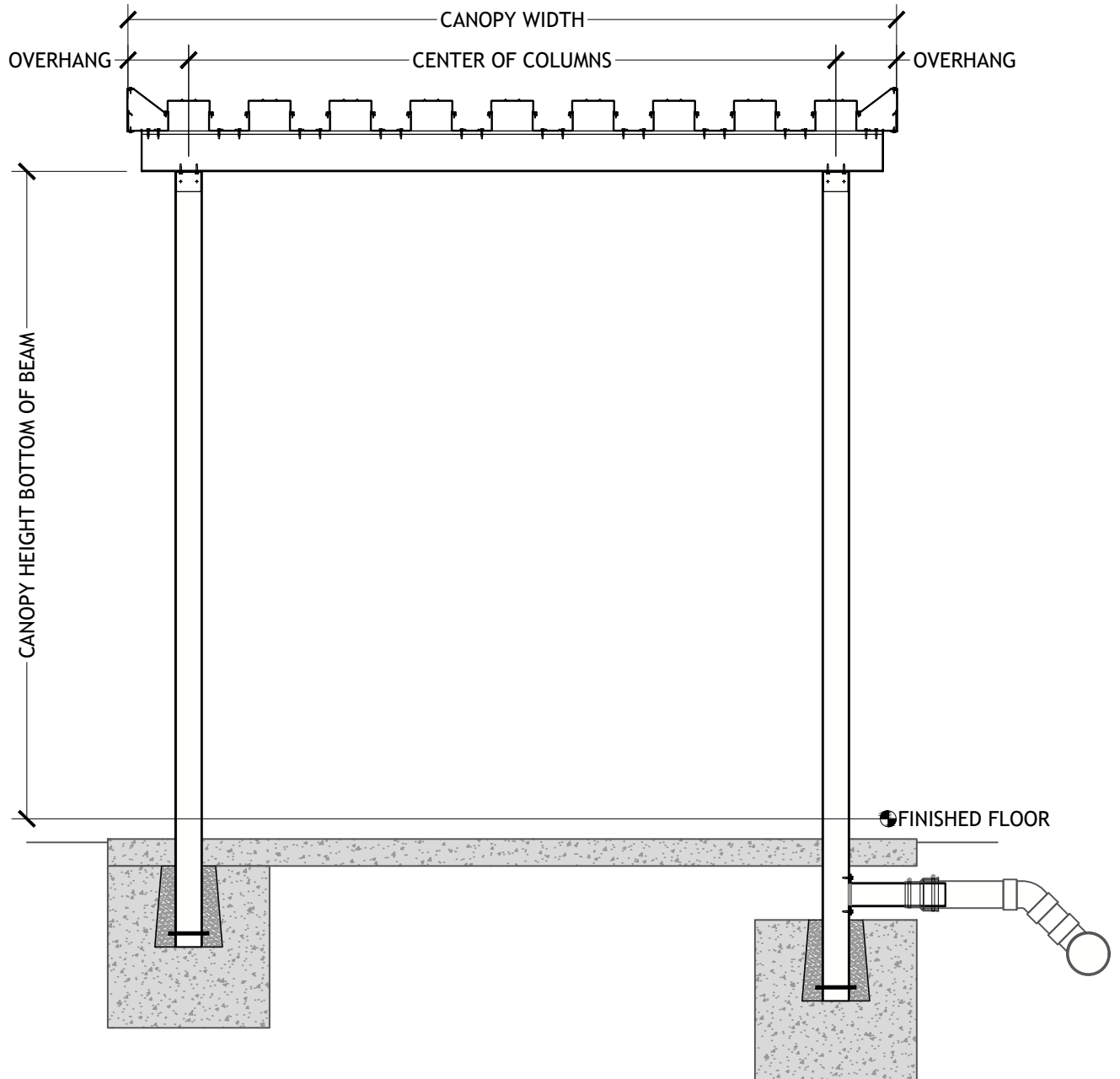
TWO POST LONG SPAN HIGH PAN & CAP DECK UNDERGROUND DRAIN
