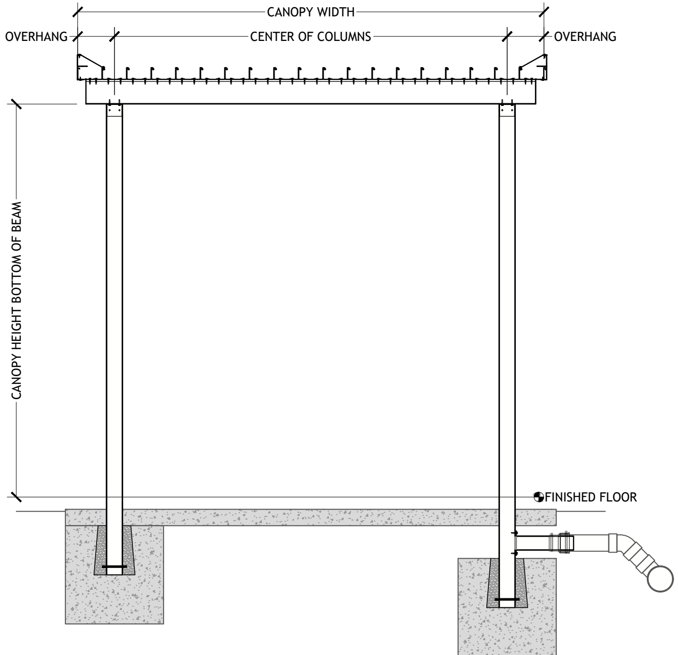
TWO POST LONG SPAN FLUSH DECK UNDERGROUND DRAIN
