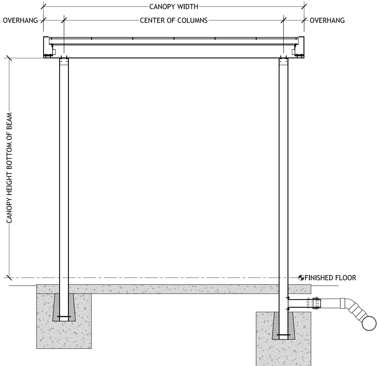
TWO POST SHORT SPAN PAN & CAP DECK UNDERGROUND DRAIN
