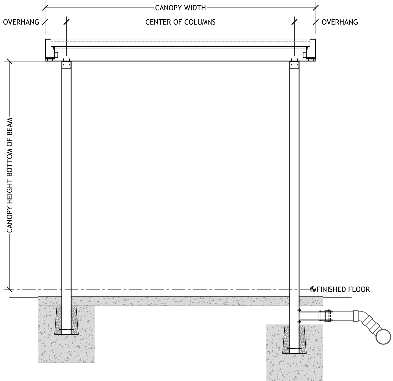
TWO POST SHORT SPAN FLUSH DECK UNDERGROUND DRAIN
